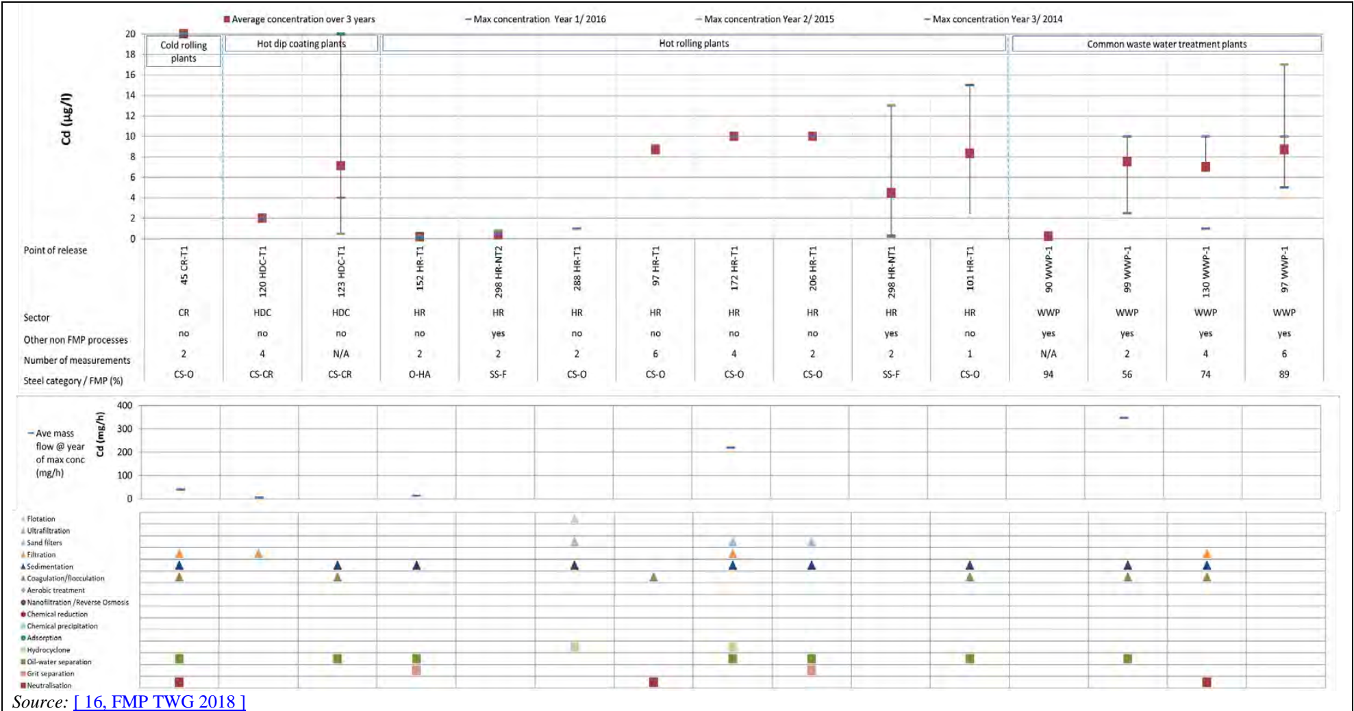
Figure 7.7: Cadmium emissions (in µg/l) for indirect discharges
