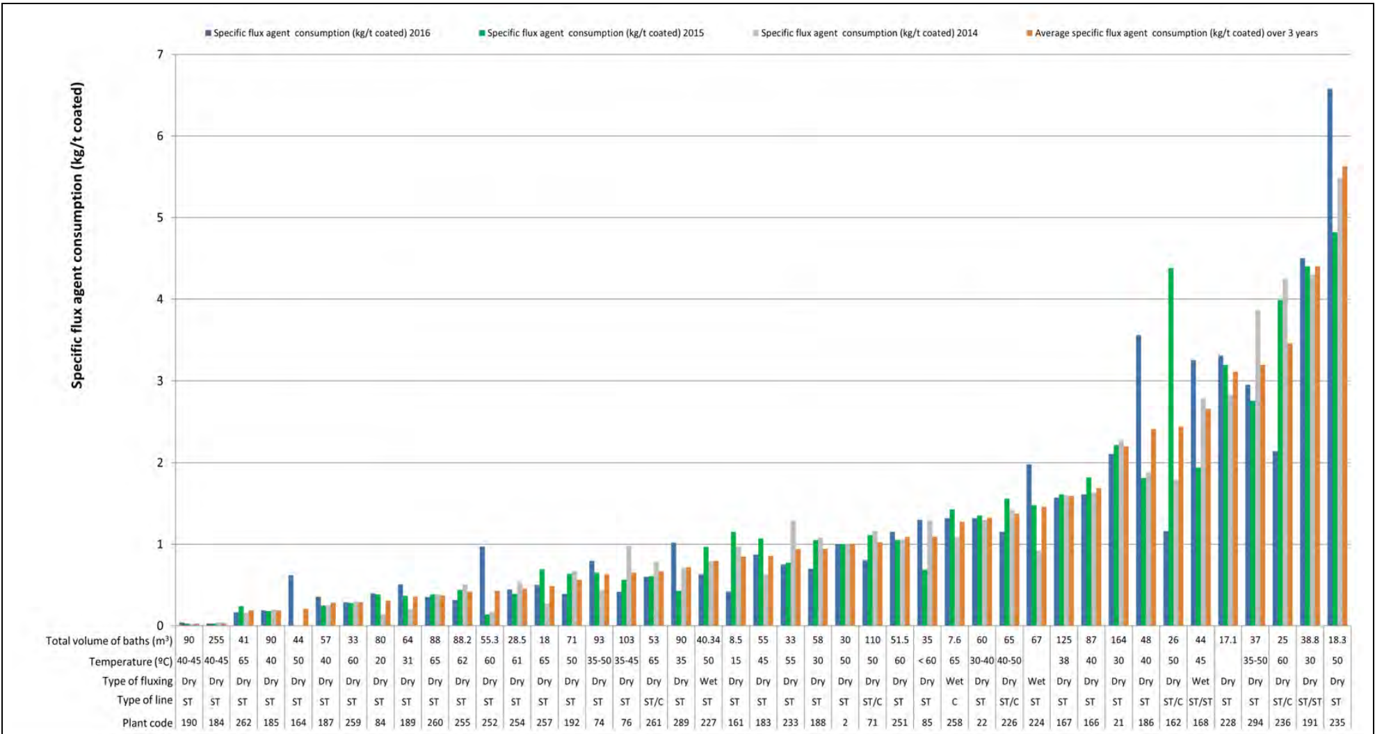
Figure 6.11: Specific flux agent consumption (kg/t of steel coated) in pickling in batch galvanising plants
