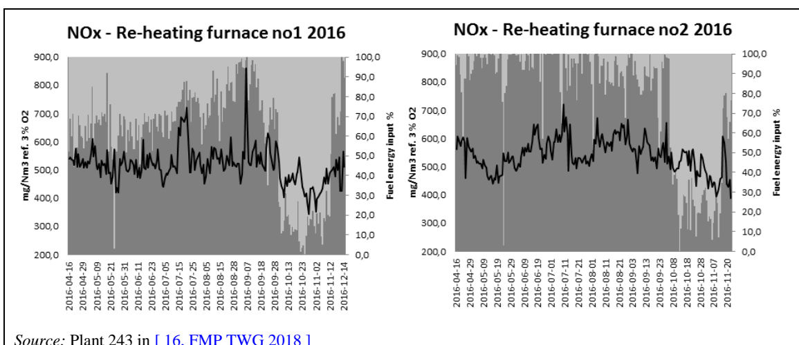
Figure 2.44: \text{NO}_x emission concentrations as a function of the type of fuels used in the reheating furnace (COG and HFO)
