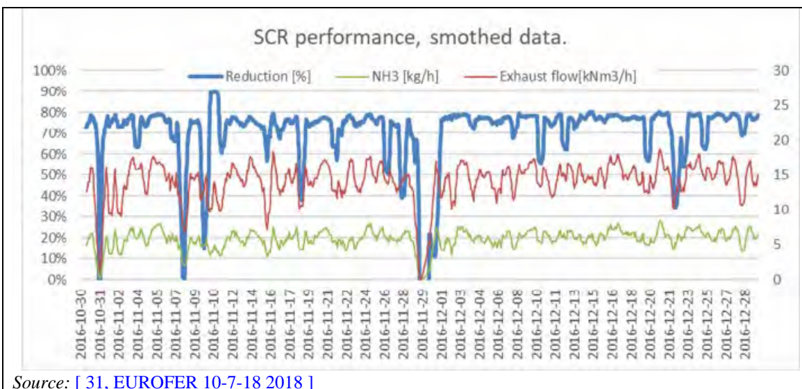
Figure 3.61: Abatement efficiency of the SCR system (%), ammonia consumption expressed in kg/h and exhaust gas flow rates expressed in kNm 3 /h at SSAB Borlänge cold rolling mill (Sweden)
