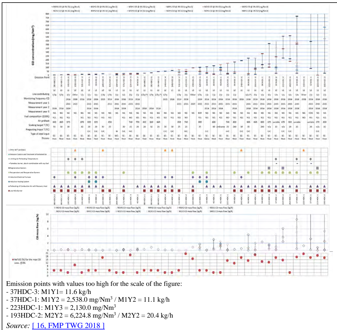
Figure 5.20: CO emissions from feedstock heating of sheet and wire (in mg/Nm³ at 3 % oxygen)
