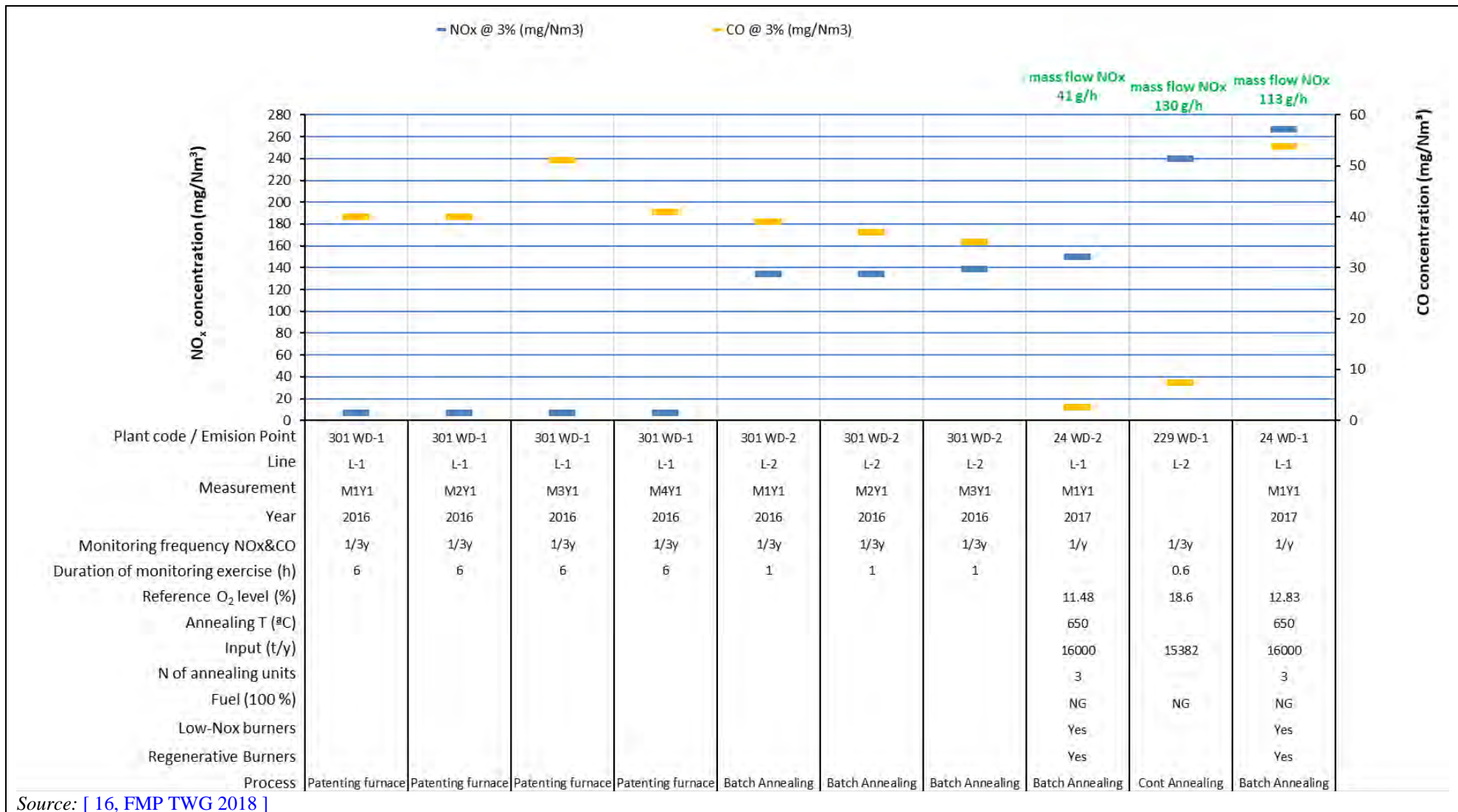
Figure 4.9: NOx and CO emissions from feedstock heating
