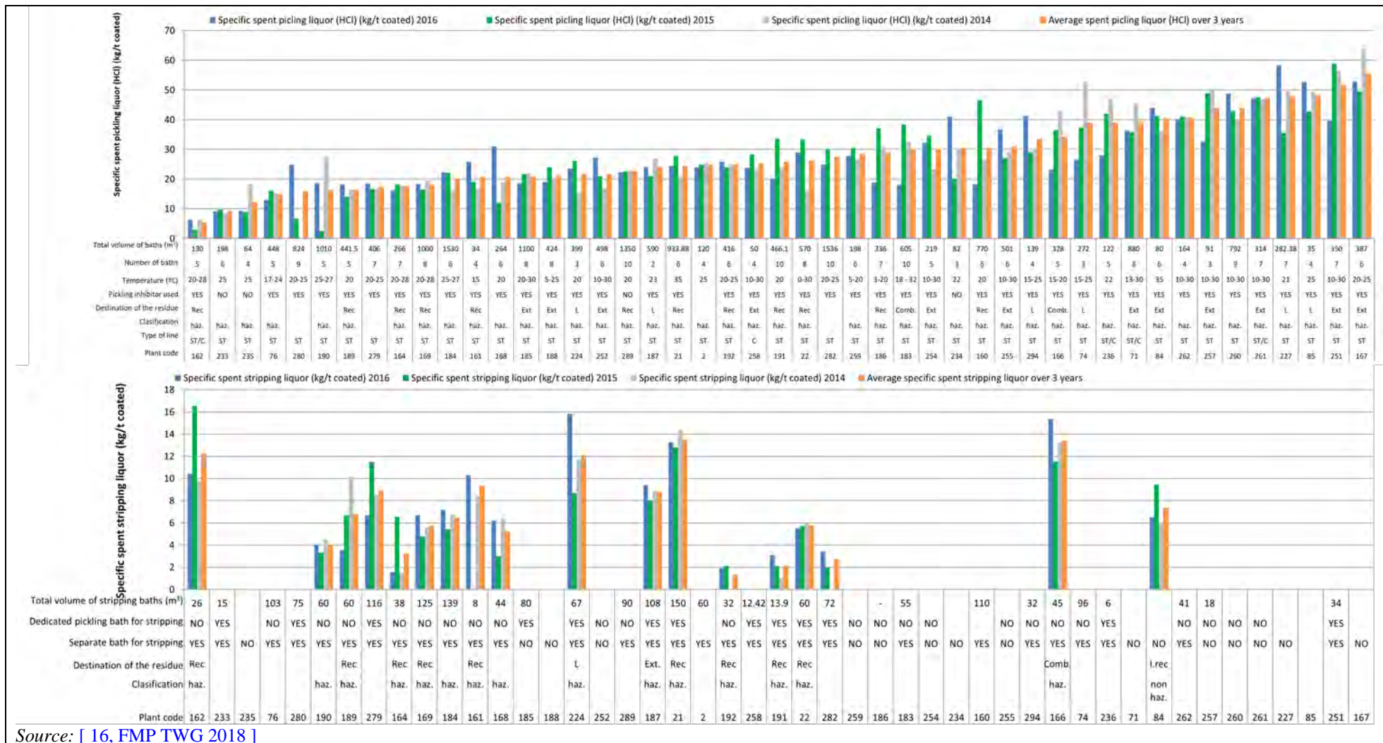
Figure 6.20: Specific generation of spent HCl from pickling and stripping (in kg/t)
