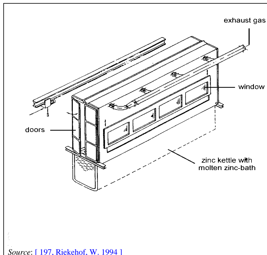
Figure 8.51: Stationary enclosure
