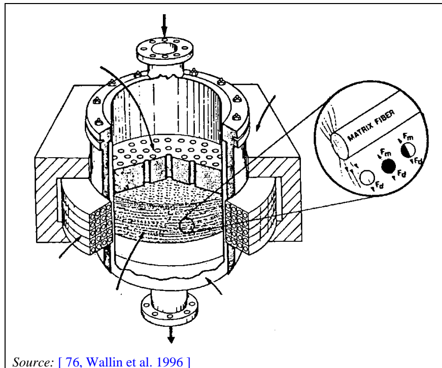
Figure 2.109: Magnetic filtration (example high gradient MF)
