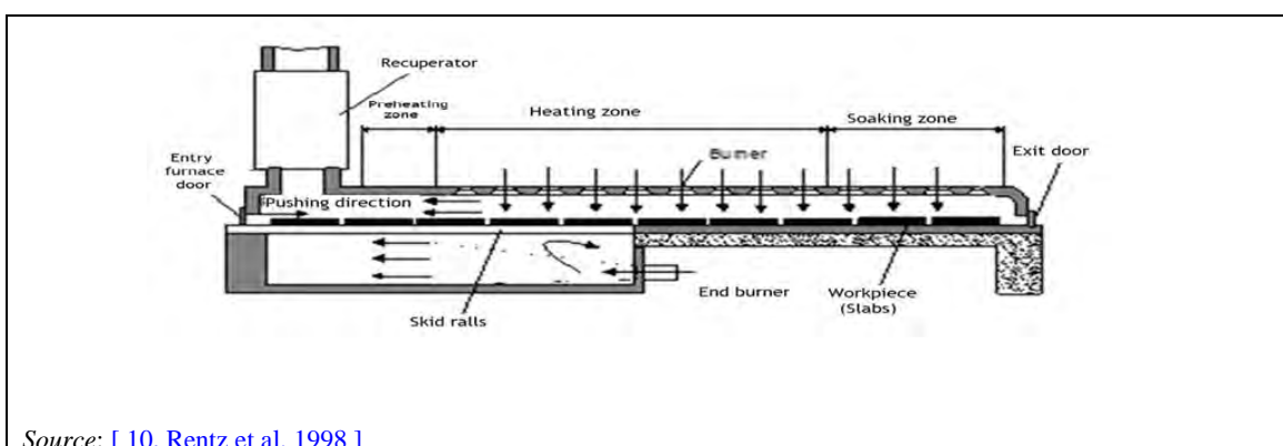
Figure 2.19: Pusher-type furnace
