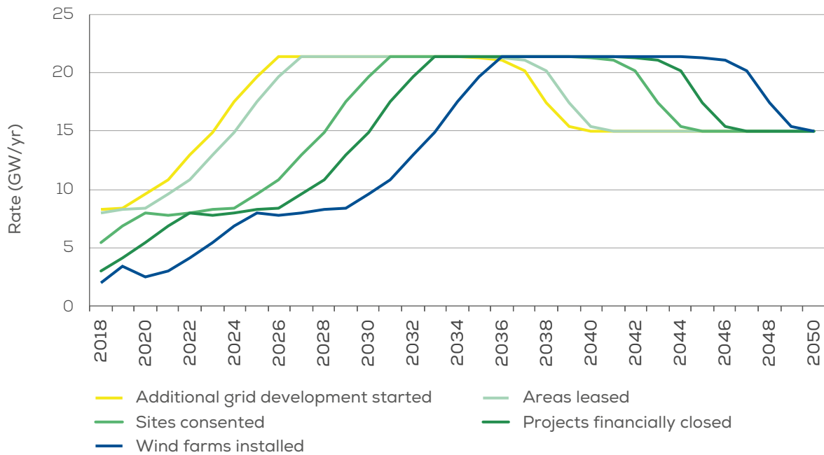
FIGURE 10 Grid development, leasing, consenting, financial closure and installation rates required to achieve 450 GW by 2050
