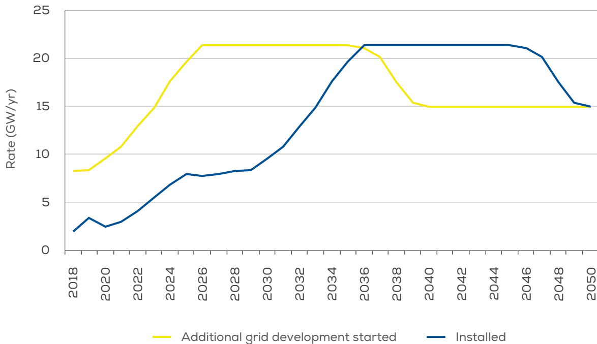
FIGURE 16 Additional grid development and installation rates required to achieve 450 GW by 2050
