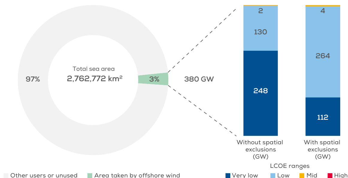
FIGURE 6 Distribution of area per sea per LCOE to allocate offshore wind in a scenario without and with spatial exclusions
