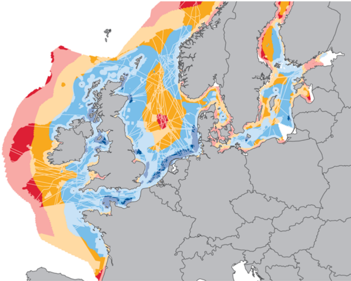
FIGURE 7 Relative LCOE for offshore wind in the North Seas (with spatial exclusions)
