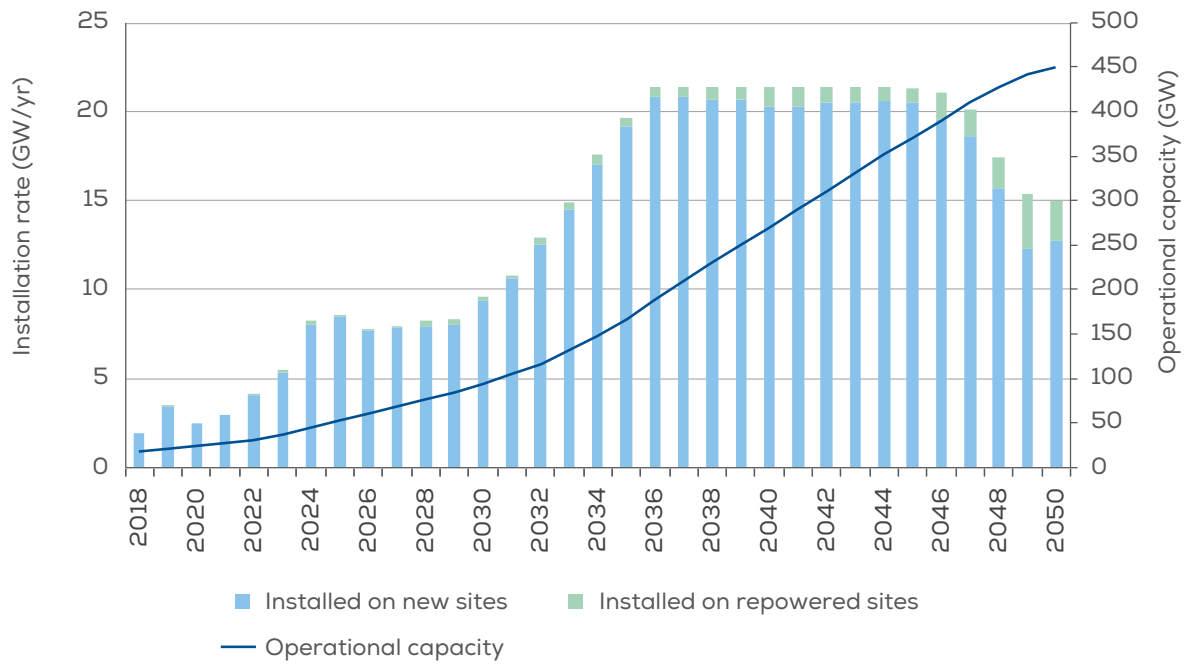
FIGURE 8 Installation rate required to achieve 450 GW by 2050
