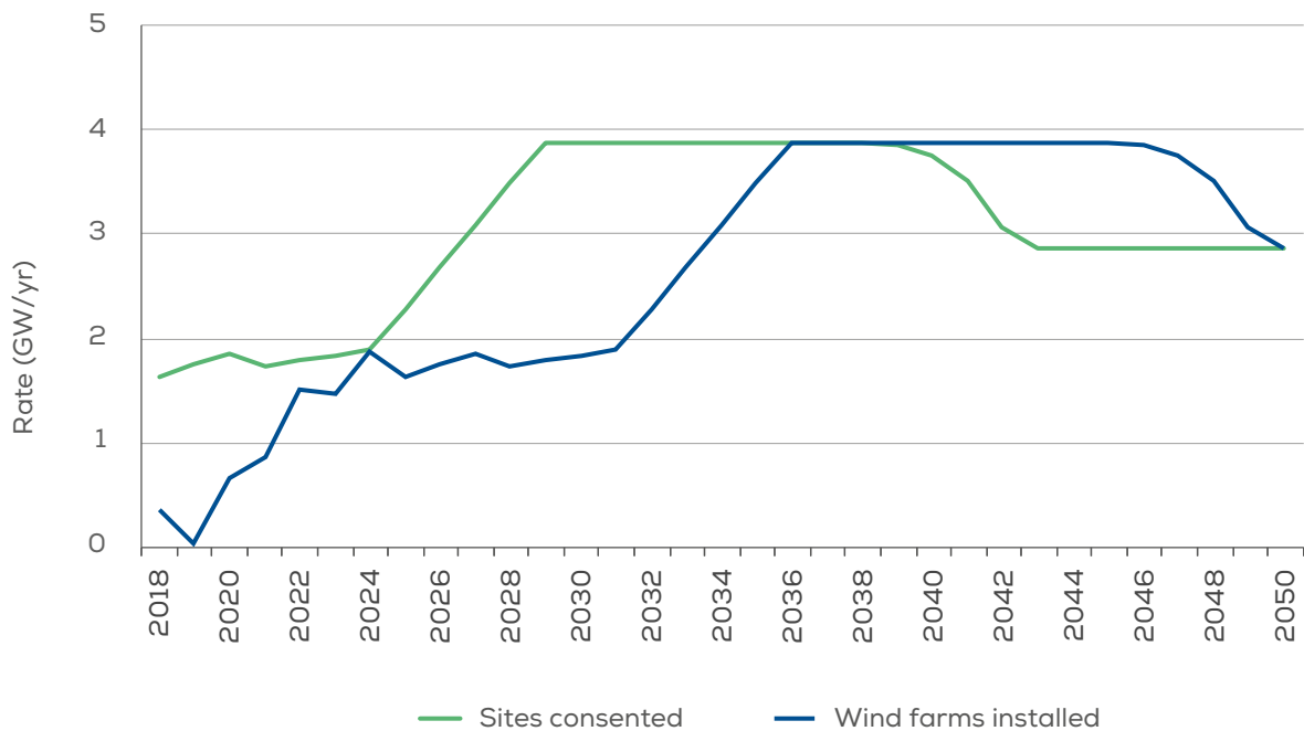
FIGURE 11 Consenting and installation rates required to achieve 85 GW by 2050 for the Atlantic Ocean
