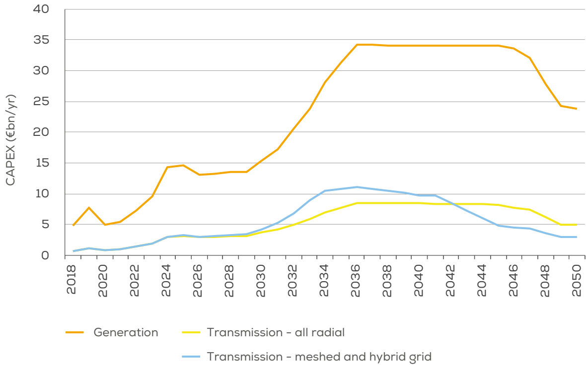
FIGURE 17 CAPEX rates required to achieve 450 GW by 2050
