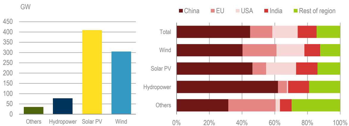
Figure 21. Renewables capacity growth in G20 countries, 2017-22
