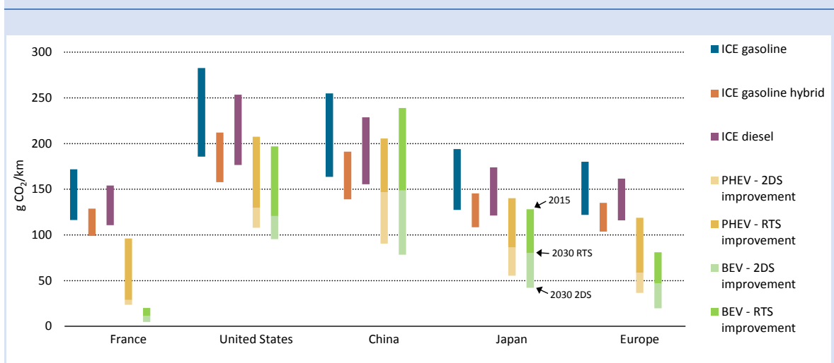
Figure 10 • On-road well-to-wheel CO 2 emissions for PLDVs for various powertrain technologies by country or region: RTS and 2DS, 2015 to 2030
