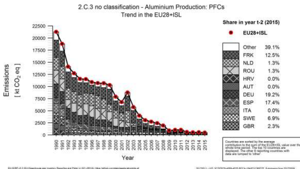
Figure 4.15 2C3 Aluminium Production: PFC emissions
