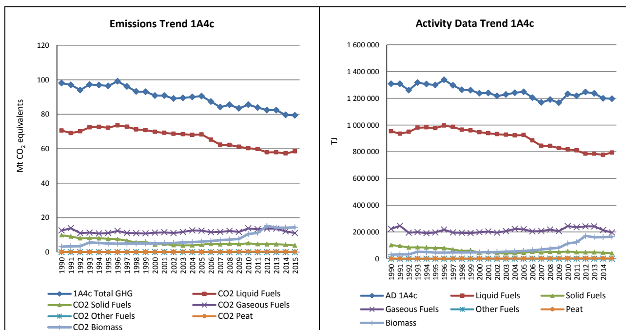
Figure 3.144 1A4c Agriculture/Forestry/Fisheries: Total and CO 2 emission trends
