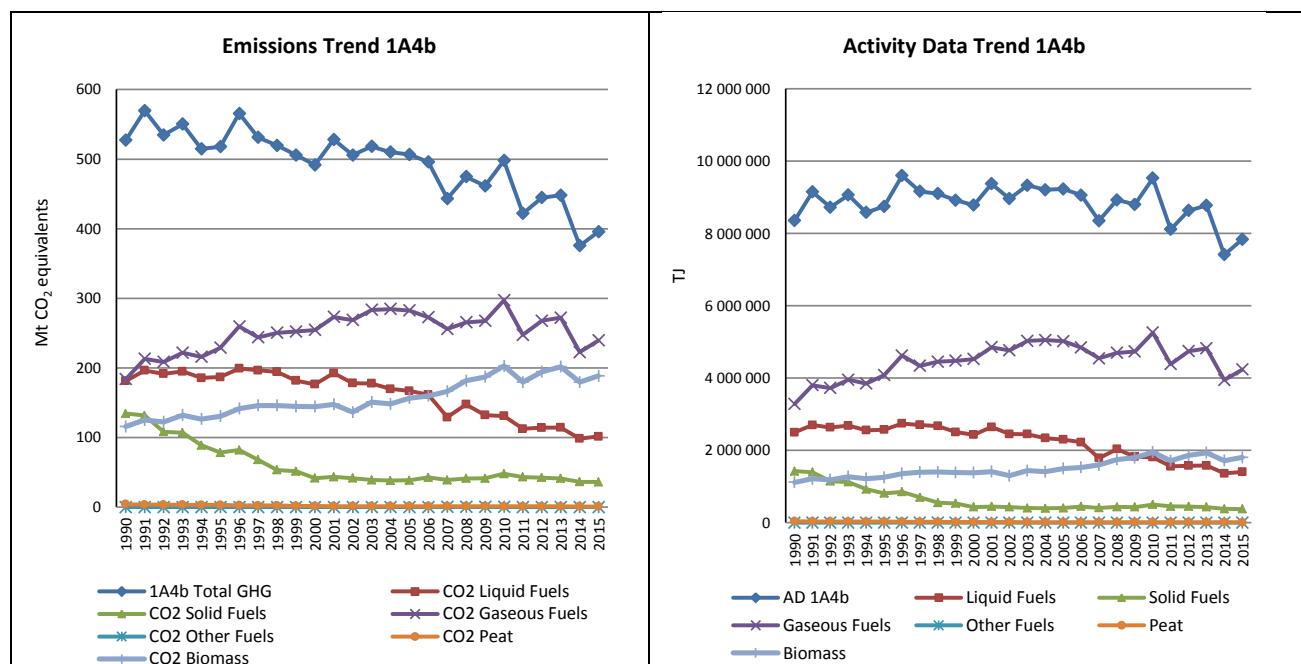
Figure 3.134 1A4b Residential: Total, CO 2 and CH 4 emission and activity trends
