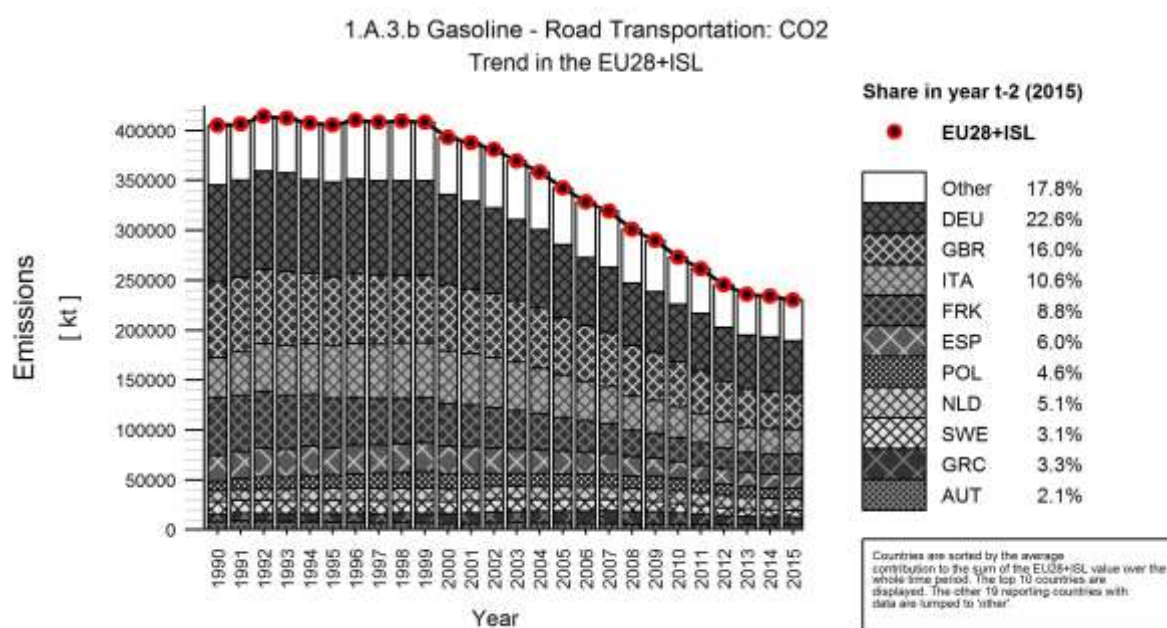
Figure 3.100 1A3b Road Transport, Gasoline: Emission trend and share for CO 2
