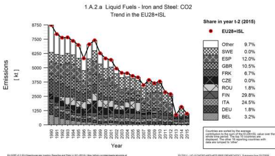
Figure 3.36 1A2a Iron and Steel, Liquid fuels: Emission trend and share for CO 2
