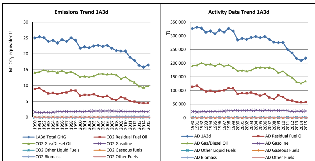
Figure 3.117 1A3d Navigation: CO 2 Emission Trend and Activity Data
