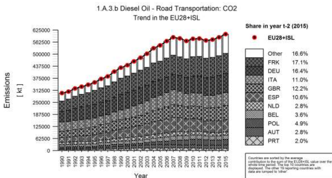
Figure 3.97 1A3b Road Transport, Diesel Oil: Emission trend and share for CO 2
