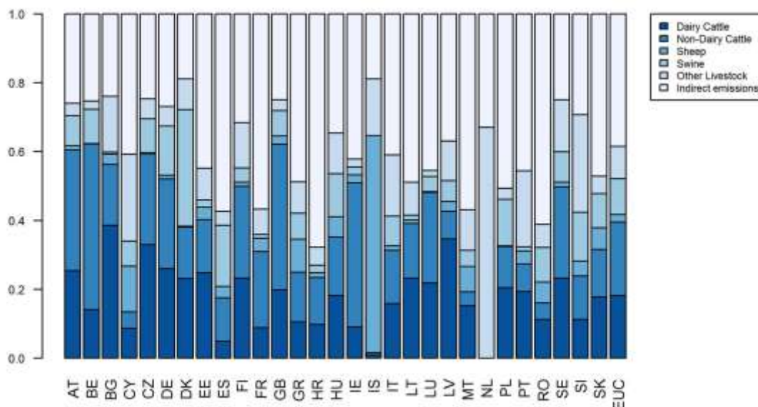
Figure 5.37: Decomposition of emissions in source category 3.B.2 - Manure Management into its sub-categories by Member State in the year 2015.
