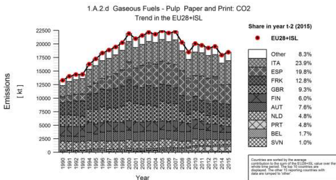
Figure 3.61 1A2d Pulp, Paper and Print, Gaseous fuels: Emission trend and share for CO 2
