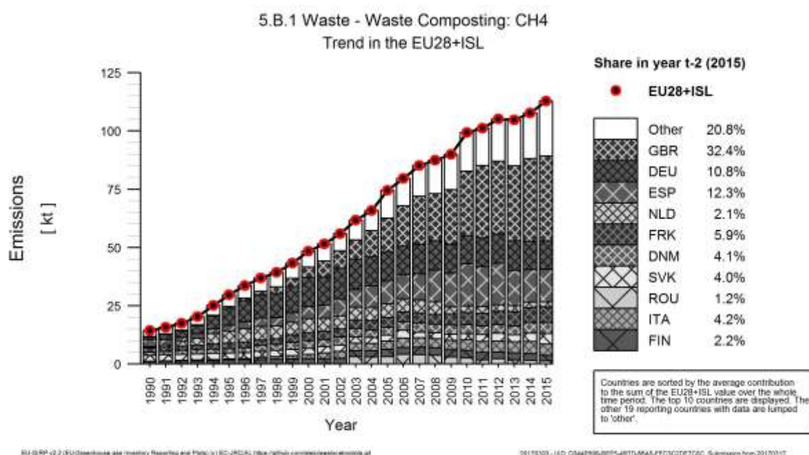
Figure 7.11 5B1 Waste Composting: CH 4 emissions (Trend in relevant MS)
