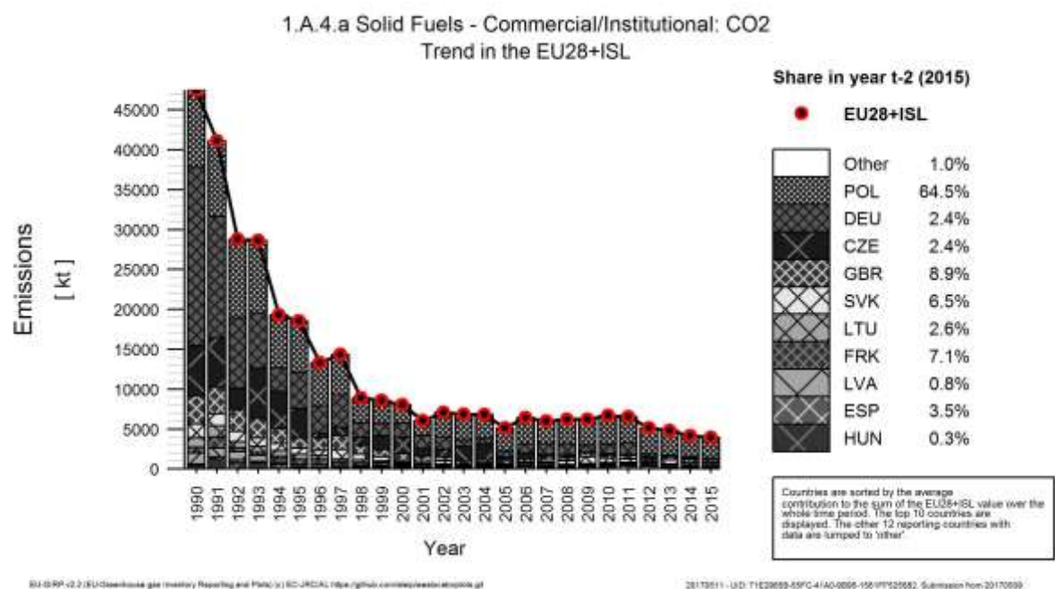
Figure 3.128 1A4a Commercial/Institutional, solid fuels: Emission trend and share for CO 2
