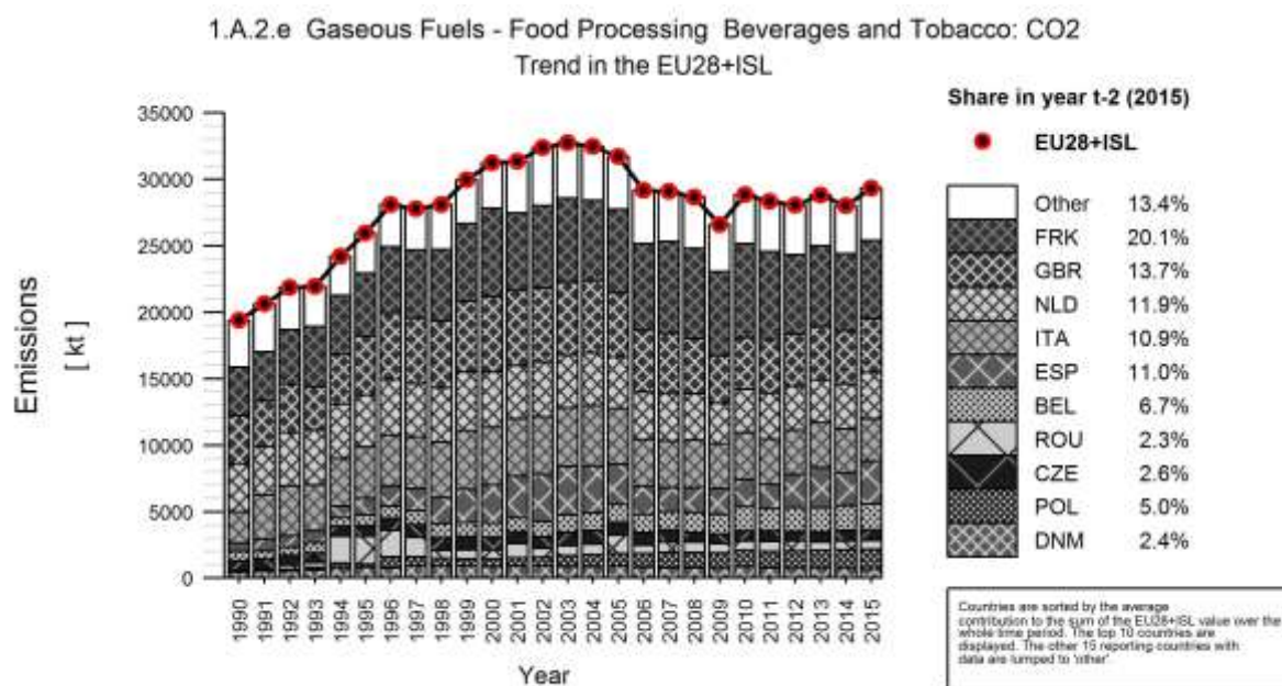
Figure 3.68 1A2e Food Processing, Beverages and Tobacco, Gaseous fuels: Emission trend and share for CO 2
