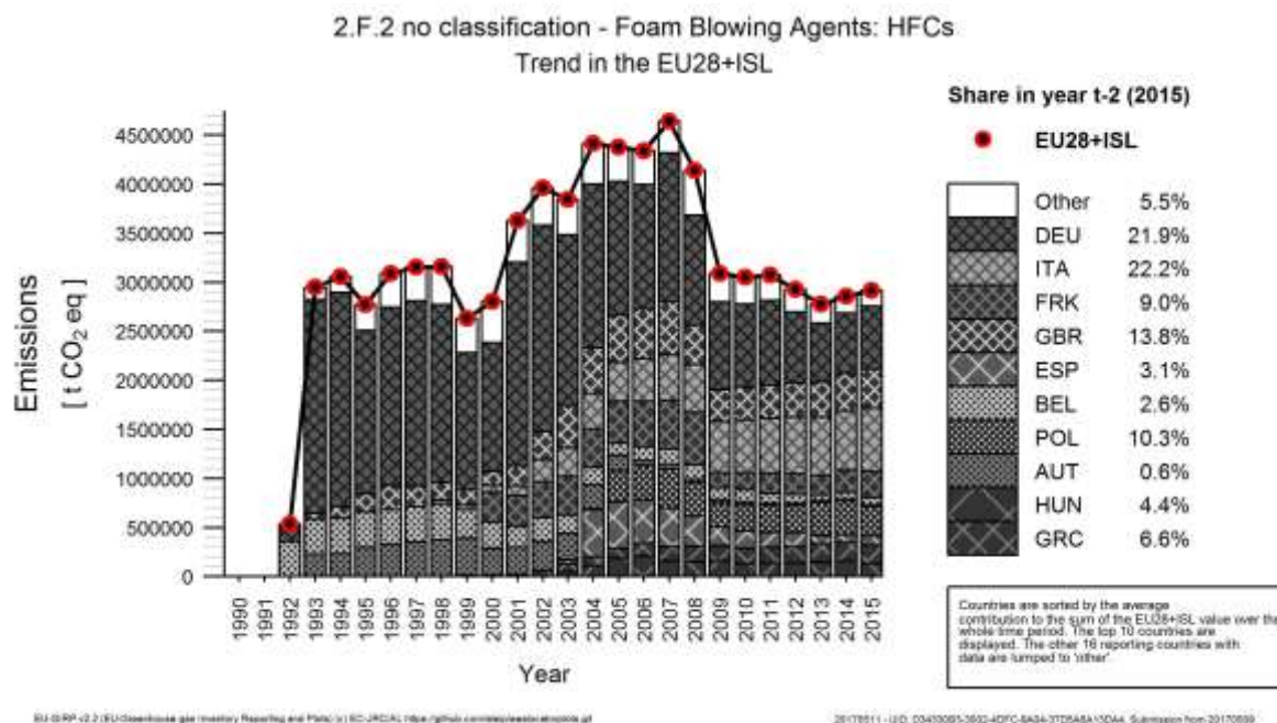
Figure 4.21: 2F2 Foam Blowing Agents: EU-28+ISL HFC emissions
