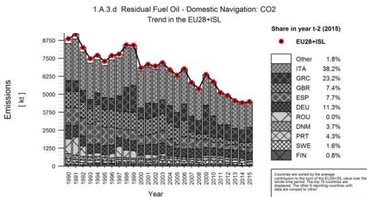
Figure 3.119 1A3d Navigation, Residual Fuel Oil: Emission trend and share for CO 2
