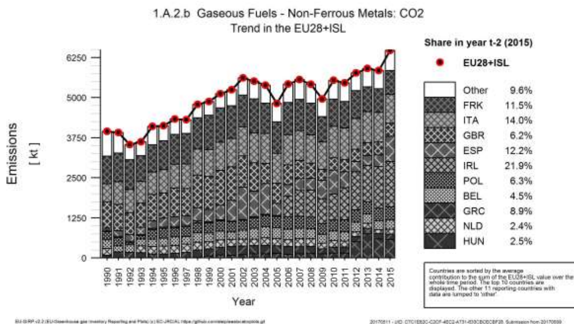
Figure 3.45 1A2b Non-ferrous Metals, Gaseous fuels: Emission trend and share for CO 2
