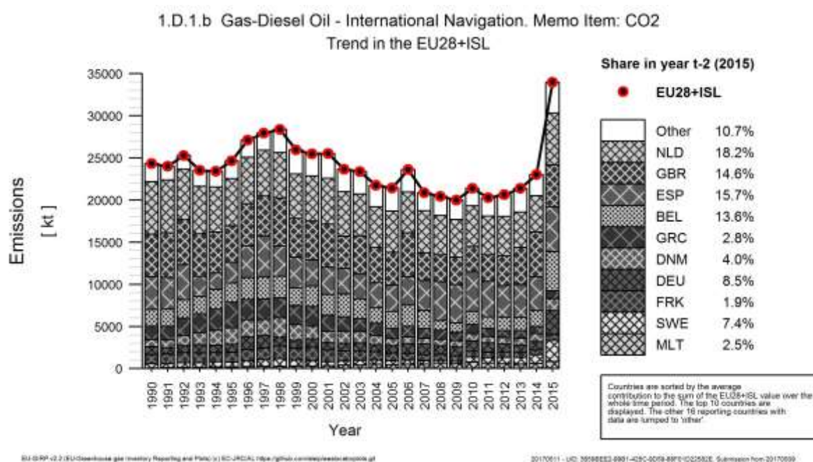
Figure 3.8 Marine bunkers, Gas/Diesel Oil: Emission trend and share for CO 2
