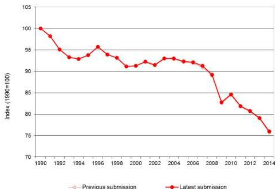
Figure 10.1: Comparison of EU-28 and Iceland GHG emission trends 1990–2014 (with indirect CO 2 , excl. LULUCF) of the latest and the previous submission
