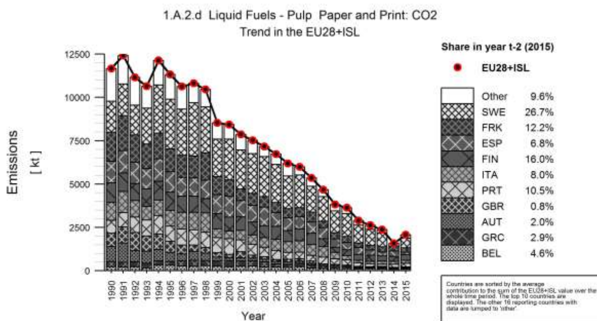
Figure 3.57 1A2d Pulp, Paper and Print, Liquid fuels: Emission trend and share for CO 2
