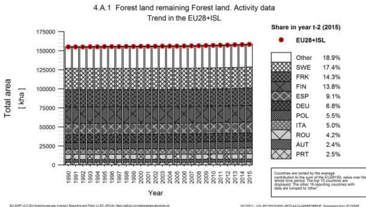
Figure 6. 3 Trend of activity data in subcategory 4A1 "Forest land remaining Forest Land" in EU MS and Iceland (kha, 1990-2015)
