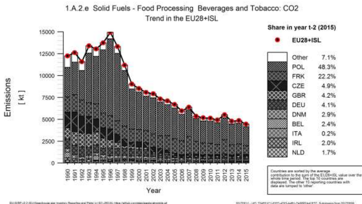
Figure 3.66 1A2e Food Processing, Beverages and Tobacco, solid fuels: Emission trend and share for CO 2
