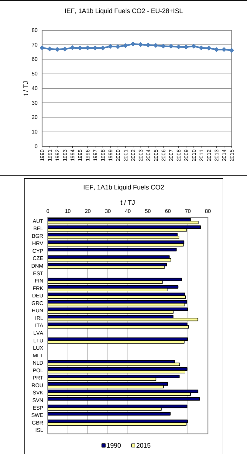
Figure 3.23 1A1b Petroleum Refining, Liquid Fuels: Implied Emission Factors for CO 2
