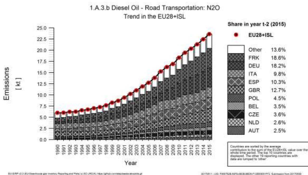
Figure 3.107 1A3b Road Transport, diesel oil: Emission trend and share for N 2 O emission
