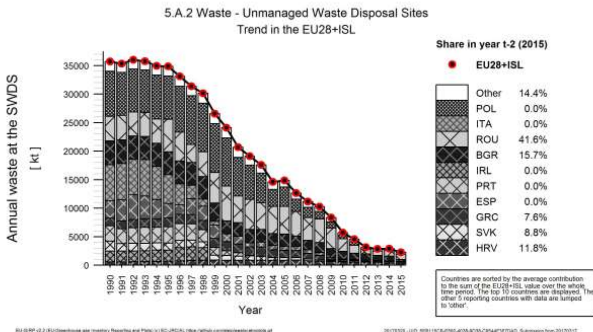
Figure 7.10 5A2 Waste disposal on unmanaged landfills: Total waste disposed on unmanaged landfills (Trend in relevant MS)
