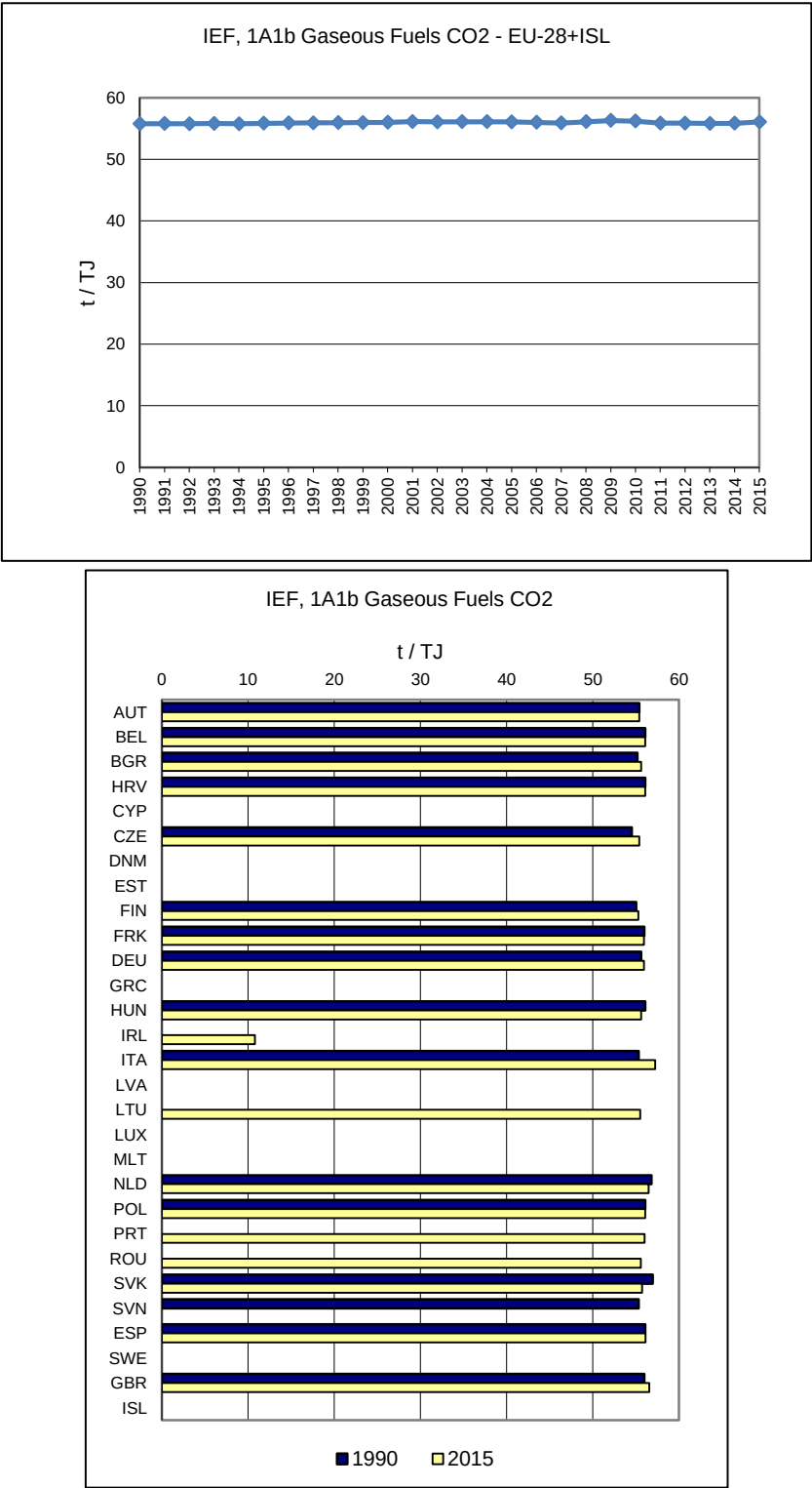
Figure 3.27 1A1b Petroleum Refining, Gaseous Fuels: Implied Emission Factors for CO 2
