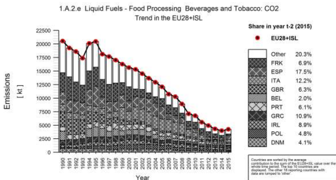
Figure 3.64 1A2e Food Processing, Beverages and Tobacco, Liquid fuels: Emission trend and share for CO 2
