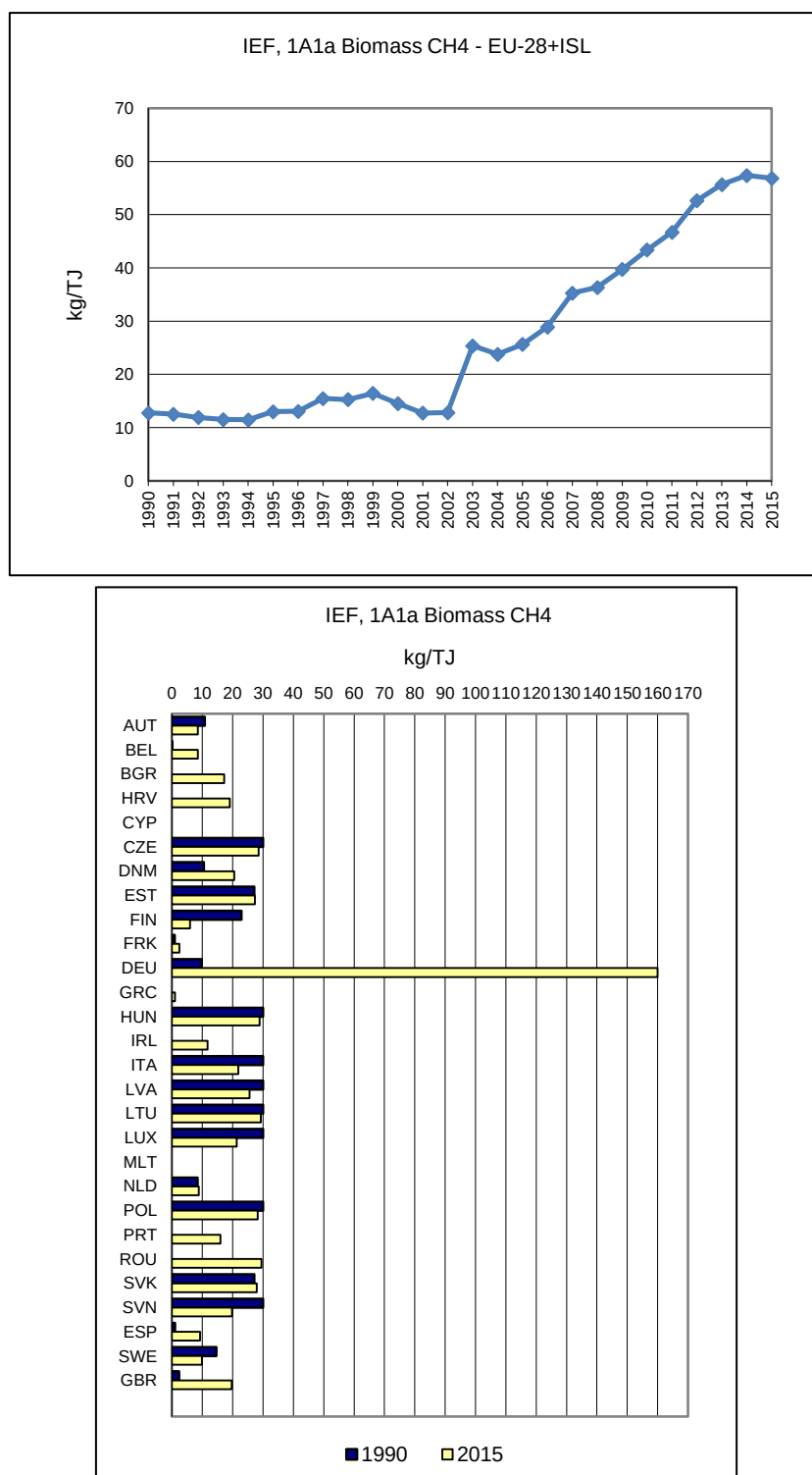
Figure 3.20 1A1a Public Electricity and Heat Production, Biomass: Implied Emission Factors for CH 4
