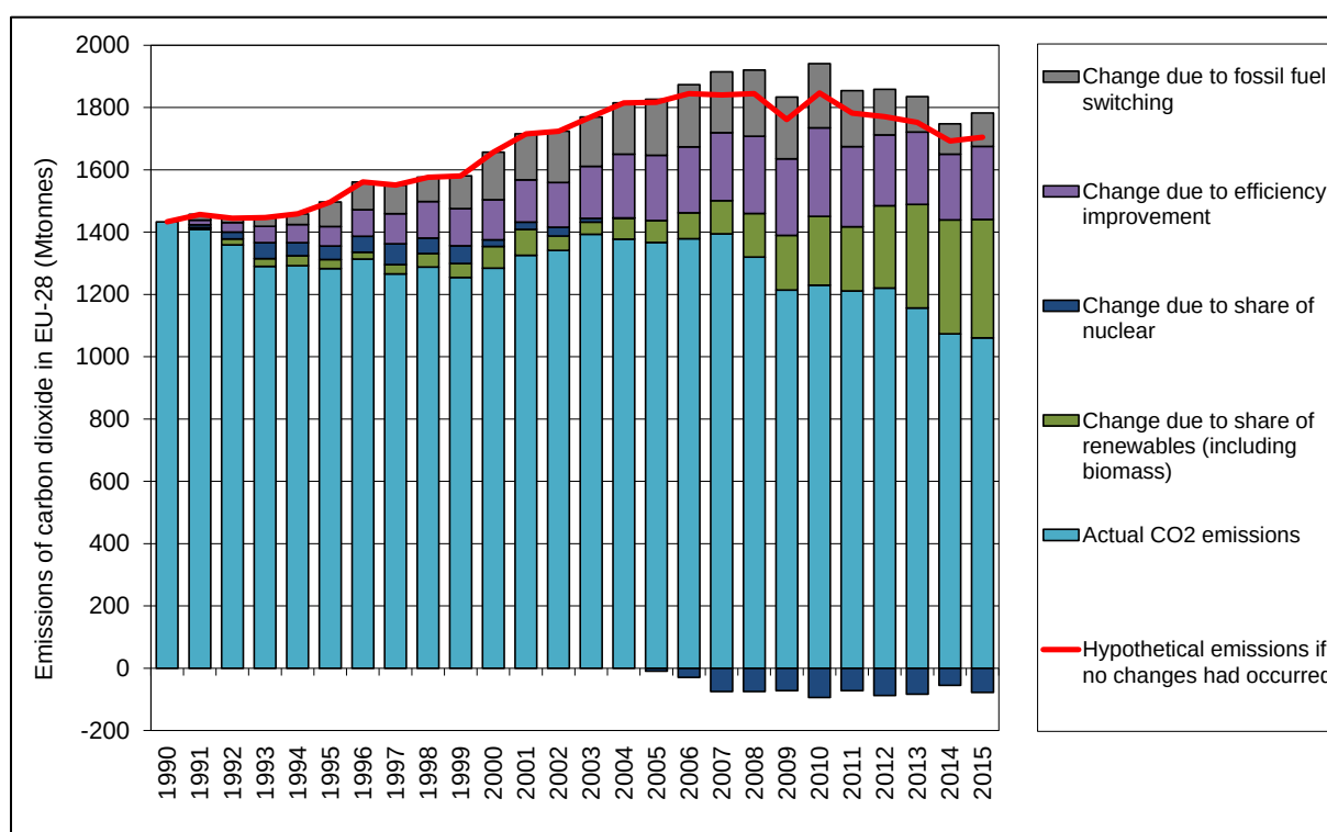
Figure 3.6 Estimated impact of different factors on the reduction in emissions of CO 2 from public electricity and heat production in the EU-28 between 1990 and 2015.
