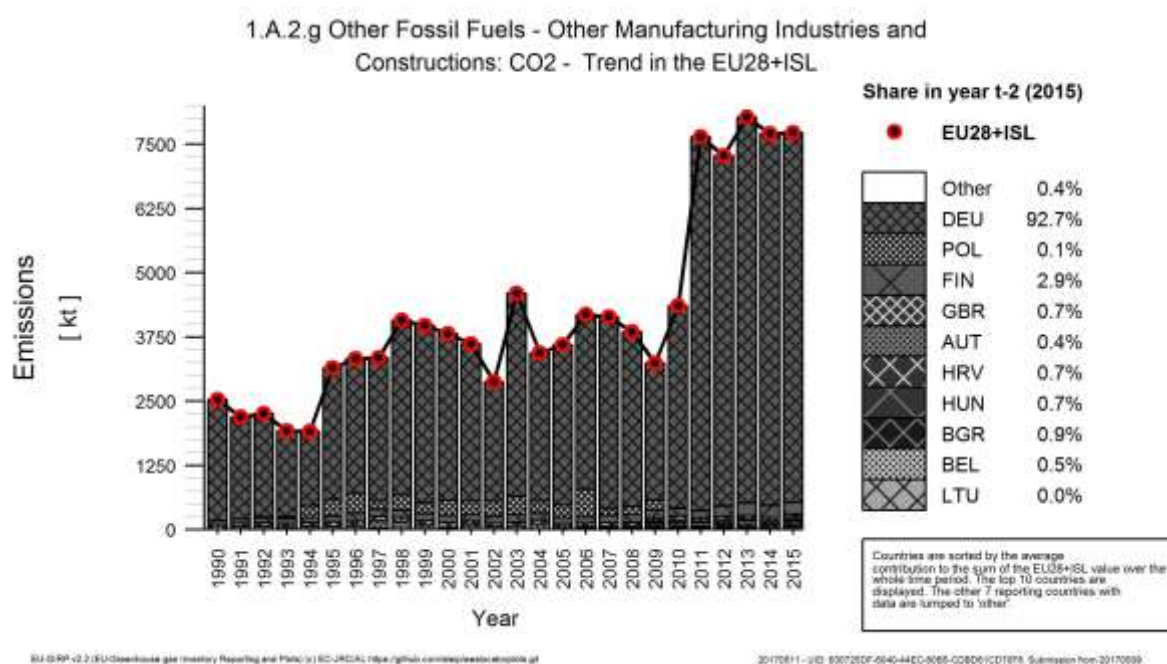
Figure 3.86 1A2g Other, other fossil fuels: Emission trend and share for CO 2
