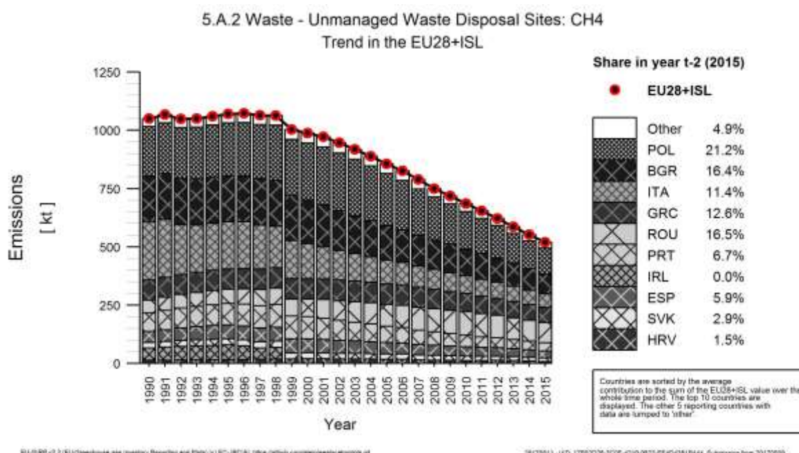
Figure 7.9 5A2 Waste disposal on unmanaged landfills: CH 4 emissions (Trend in relevant MS)
