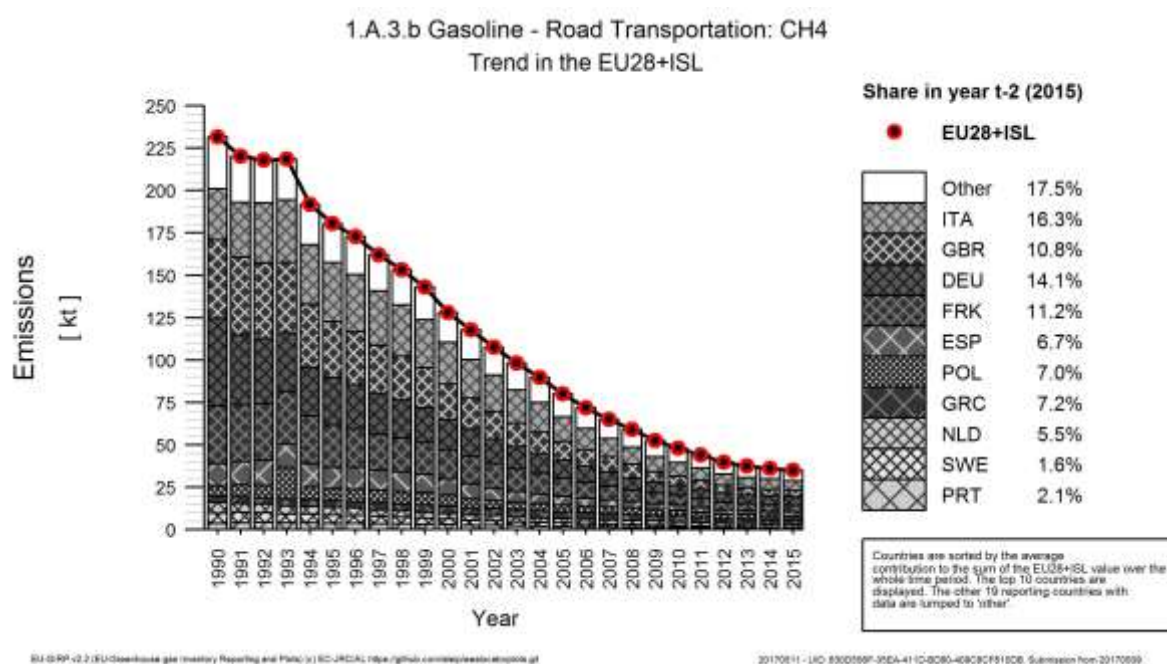
Figure 3.103 1A3b Road Transport, gasoline: Emission trend and share for CH 4 emission
