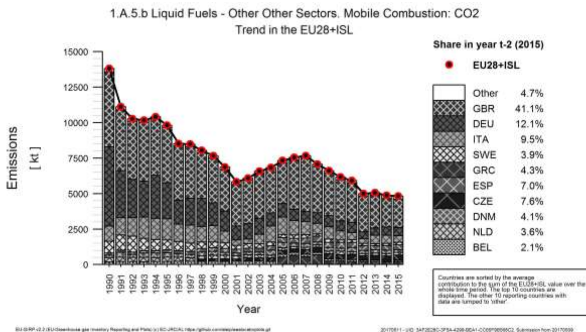
Figure 3.156 1A5b Mobile, liquid fuels: Emission trend and share for CO 2
