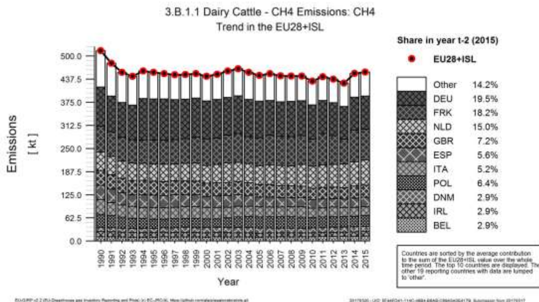
Figure 5.24: 3.B.1.1: Trend in emissions in the EU28+ISL and the countries contributing most to EU28+ISL values including their share to EU28+ISL emissions in 2015
