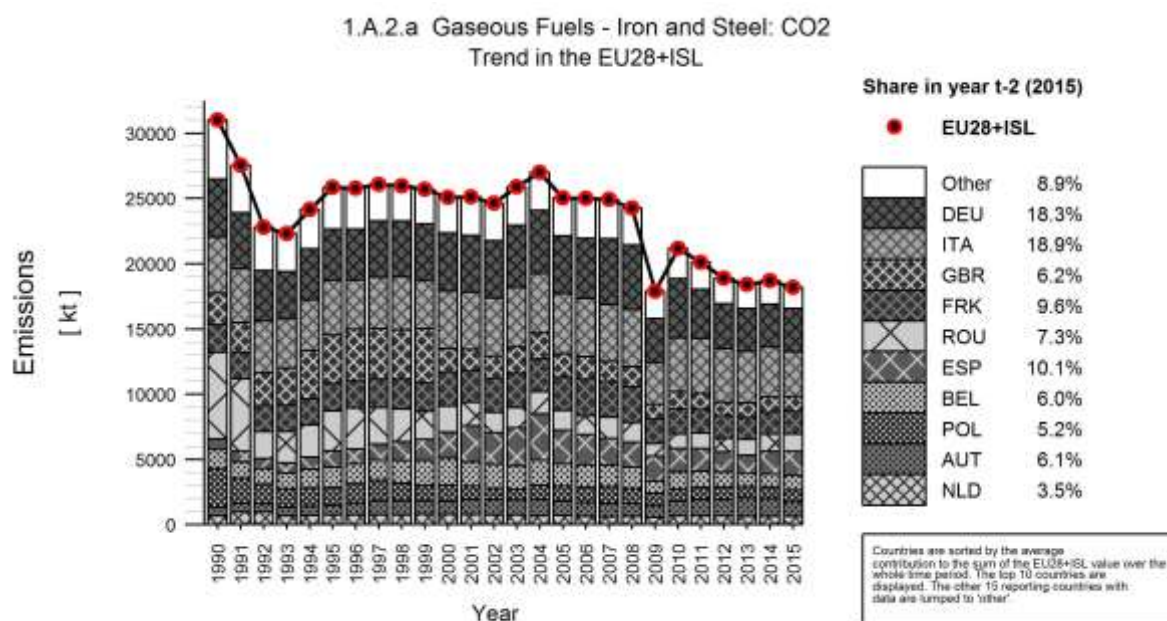
Figure 3.40 1A2a Iron and Steel, Gaseous fuels: Emission trend and share for CO 2
