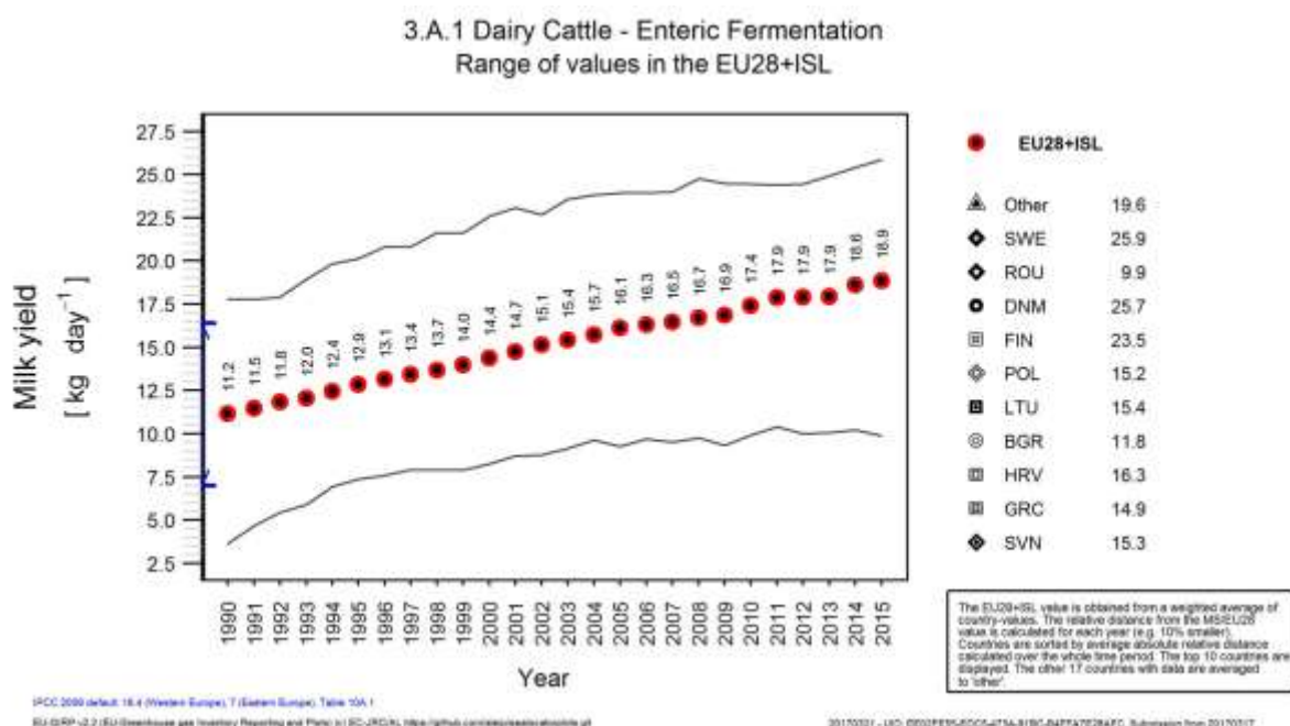
Figure 5.15: 3.A.1 - Dairy Cattle: Trend in milk yield in the EU28+ISL and range of values reported by countries
