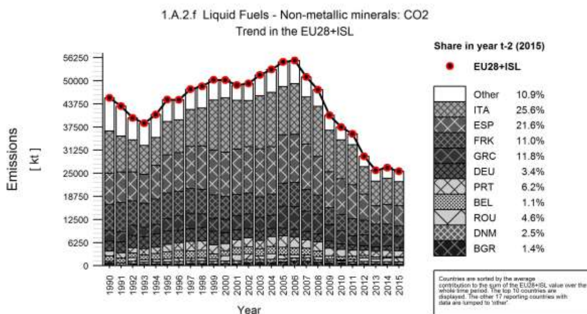
Figure 3.71 1A2f Non-metallic Minerals, liquid fuels: Emission trend and share for CO 2
