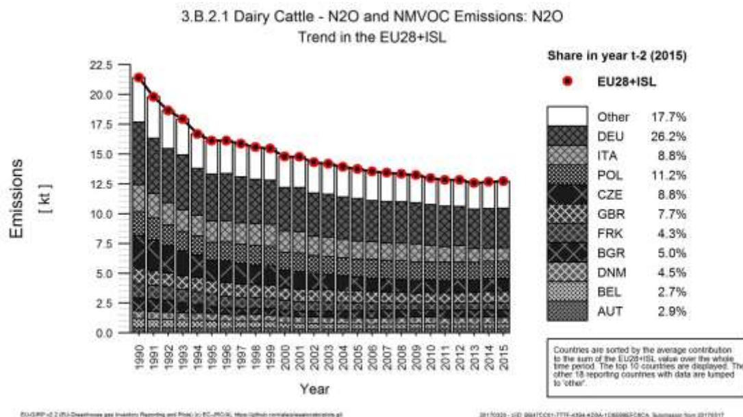
Figure 5.41: 3.B.2.1 - Cattle: Trend in emissions in the EU28+ISL and the countries contributing most to EU28+ISL values including their share to EU28+ISL emissions in 2015
