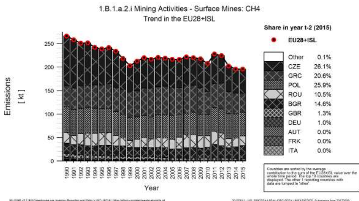
Figure 3.163 1B1a2i Mining activities - Surface Mines: Emission trend and share for the emitting countries of CH 4
