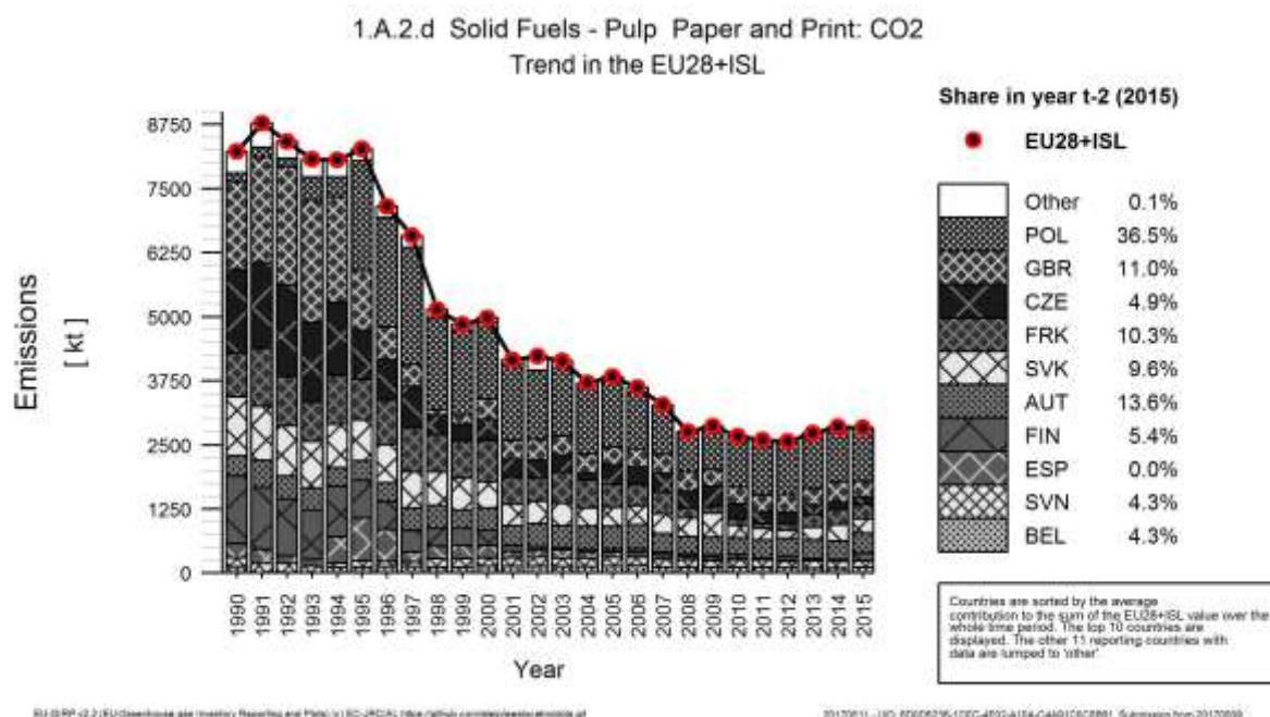
Figure 3.59 1A2d Pulp, Paper and Print, Solid fuels: Emission trend and share for CO 2
