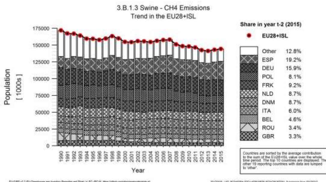
Figure 5.26: 3.B.1.3: Trend in swine population in the EU28+ISL and the countries contributing most to EU28+ISL values including their share to EU28+ISL emissions in 2015
