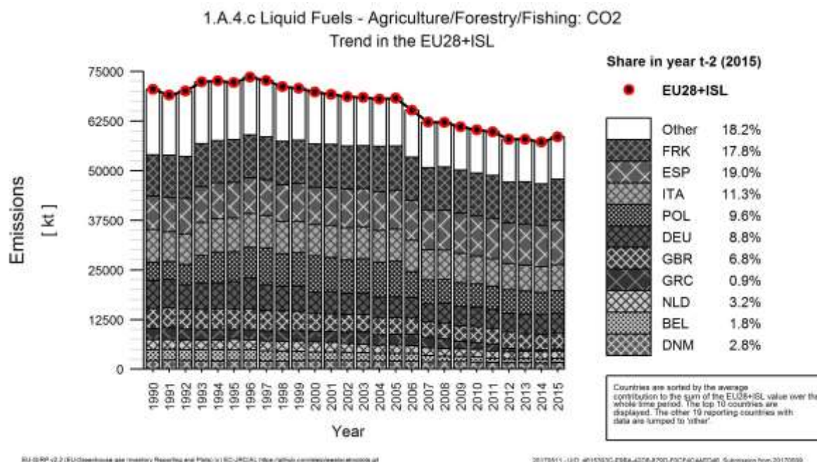
Figure 3.145 1A4c Agriculture/Forestry/Fisheries, liquid fuels: Emission trend and share for CO 2
