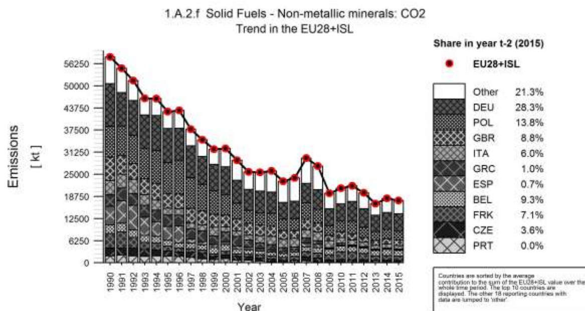
Figure 3.73 1A2f Non-metallic Minerals, solid fuels: Emission trend and share for CO 2
