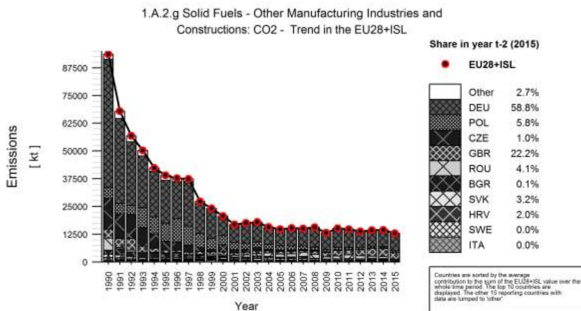
Figure 3.82 1A2g Other, solid fuels: Emission trend and share for CO 2
