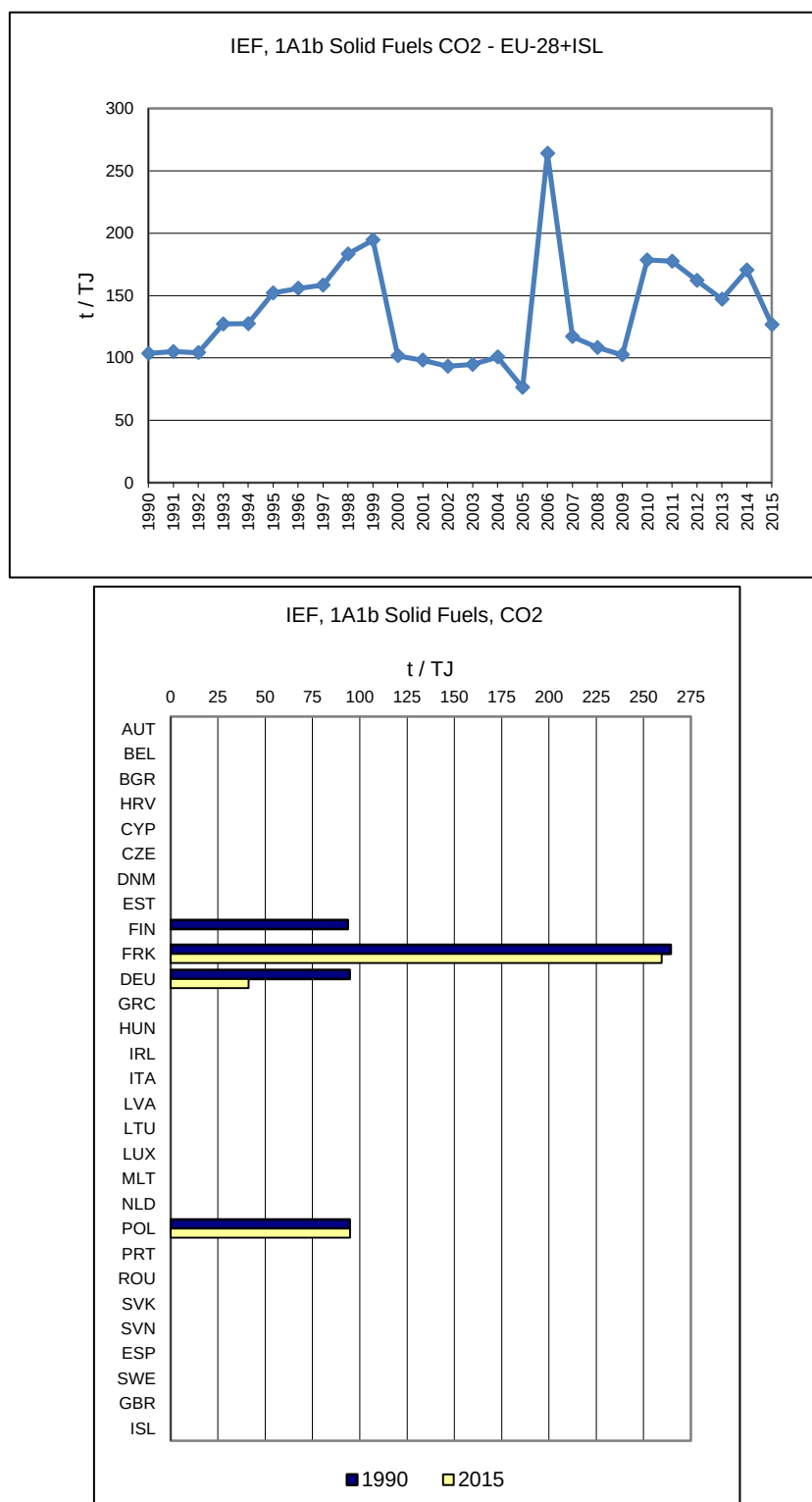
Figure 3.25 1A1b Petroleum Refining, Solid Fuels: Implied Emission Factors for CO 2
