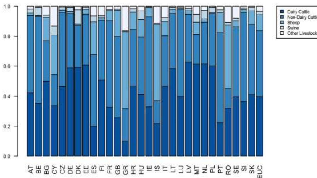
Figure 5.5: Decomposition of emissions in source category 3.A - Enteric Fermentation into its sub-categories by Member State in the year 2015.
