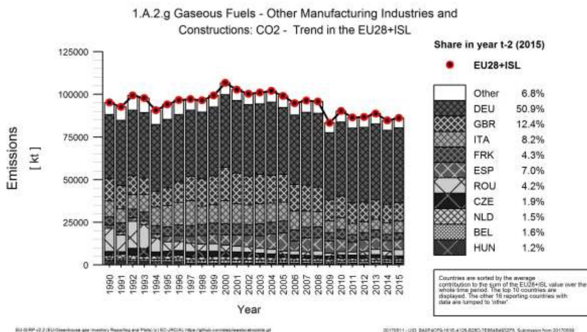
Figure 3.84 1A2g Other, gaseous fuels: Emission trend and share for CO 2
