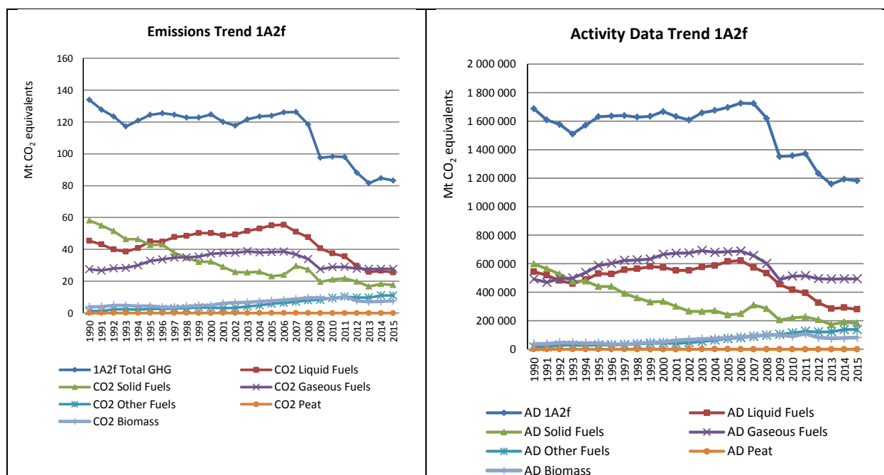
Figure 3.70 1A2f Non-metallic Minerals: Activity data and CO 2 emission trends
