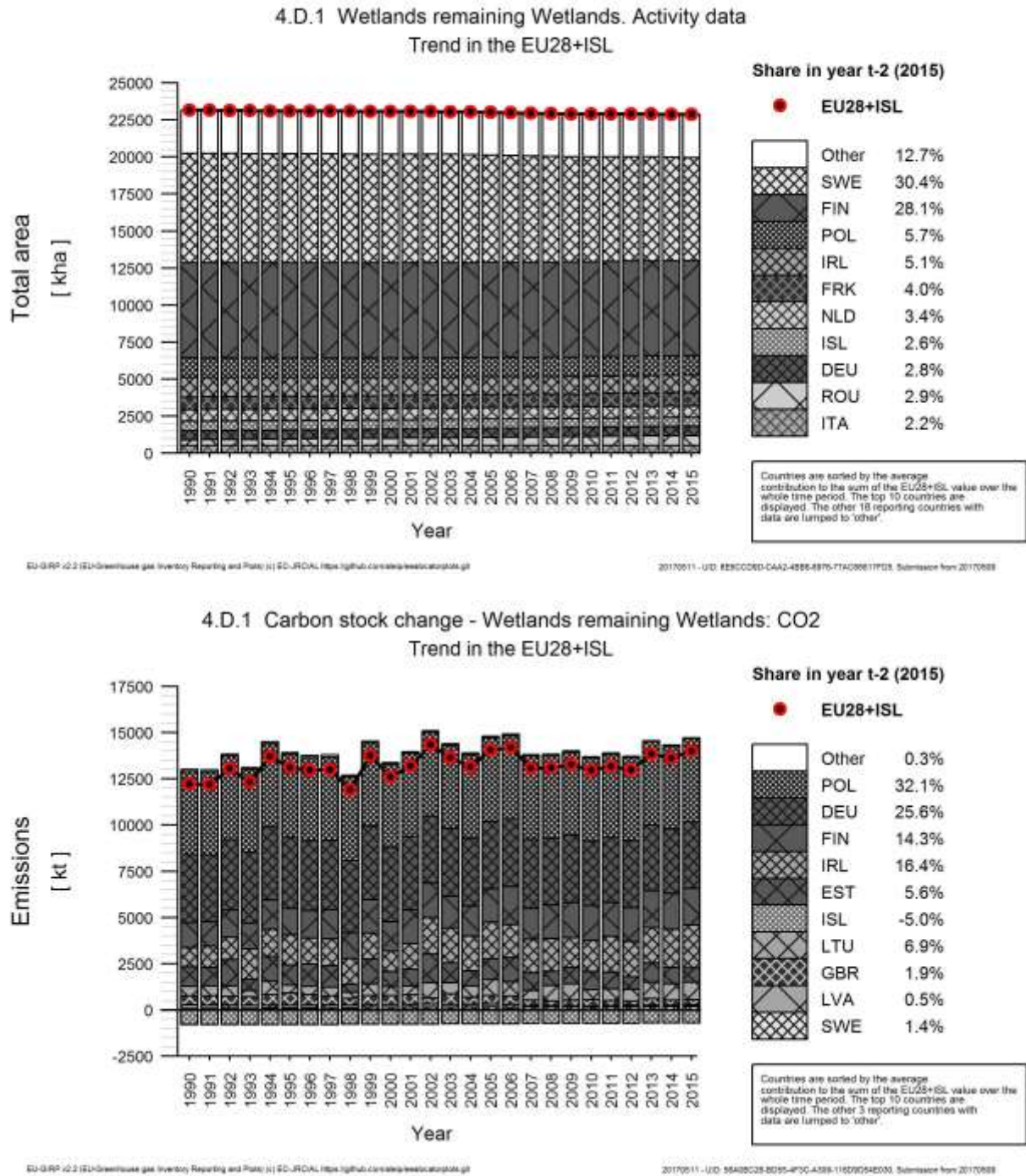
Figure 6. 15 Trend of activity data and emissions (+)/removals (-) in subcategory 4D1 “Wetlands remaining Wetlands” in EU MS and Iceland (kha, Kt CO 2 , 1990-2015)
