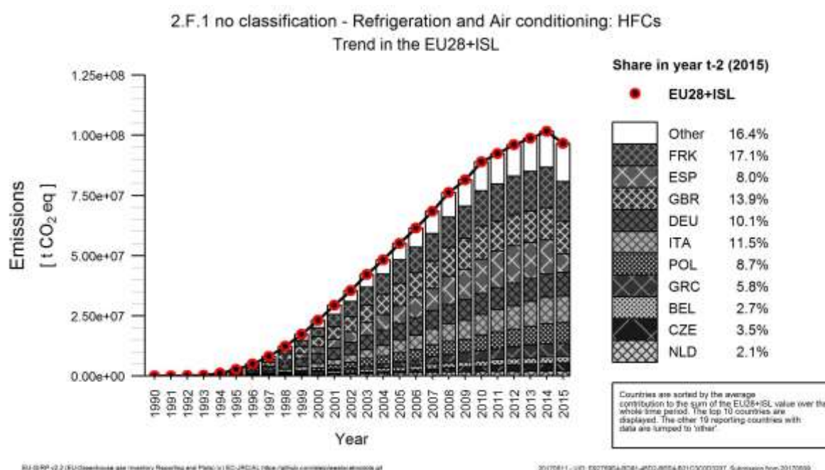
Figure 4.17: 2F1 Refrigeration and Air conditioning: EU-28+ISL HFC emissions
