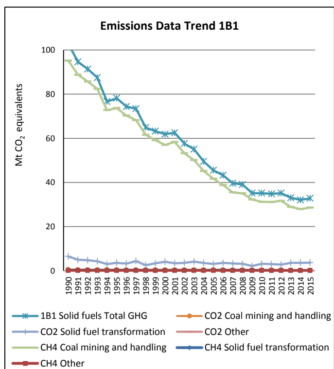
Figure 3.159 1B1 Fugitive Emissions from Solid Fuels: Trend
