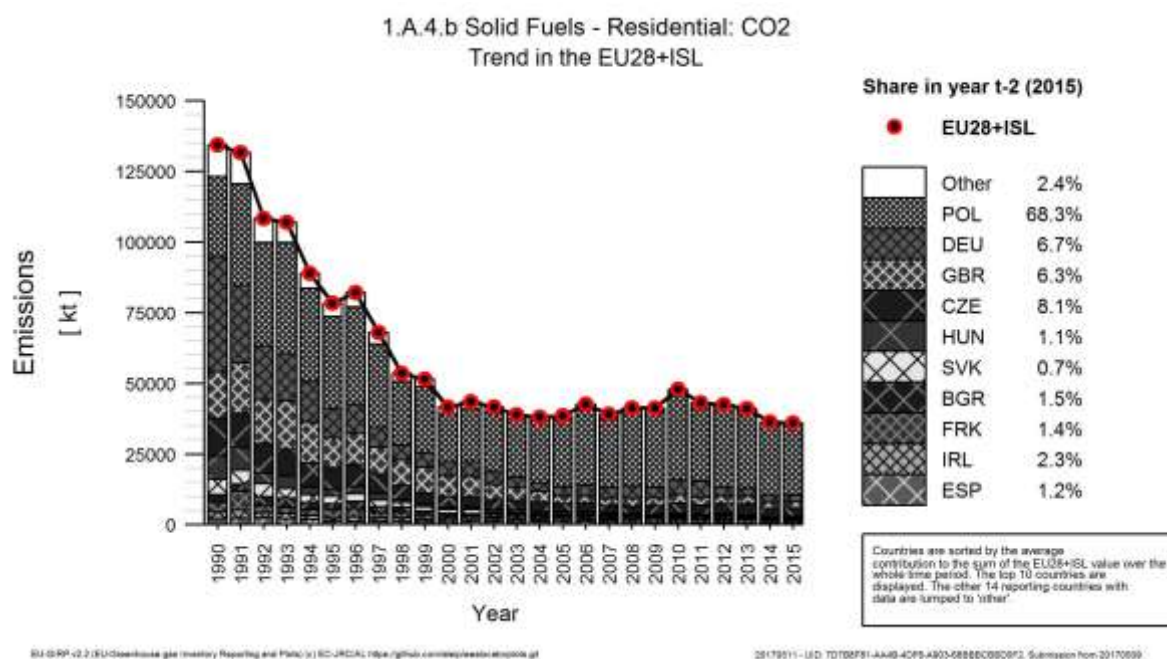
Figure 3.137 1A4b Residential, solid fuels: Emission trend and share for CO 2
