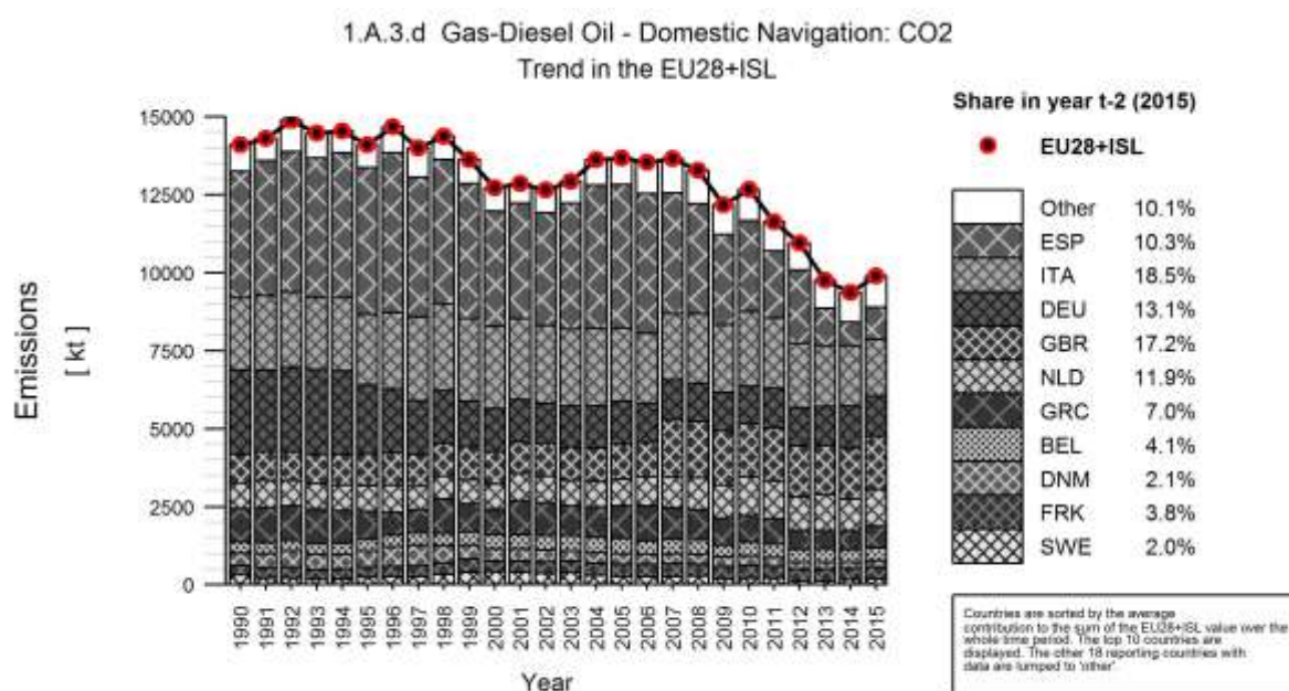
Figure 3.122 1A3d Navigation, Gas/Diesel Oil: Emission trend and share for CO 2
