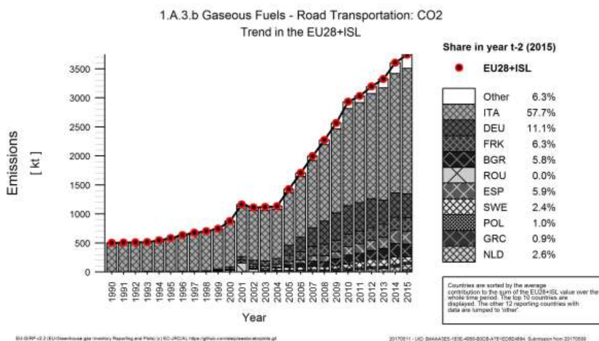
Figure 3.94: 1A3b Road Transport, gaseous fuels: Emission trend and share for CO 2
