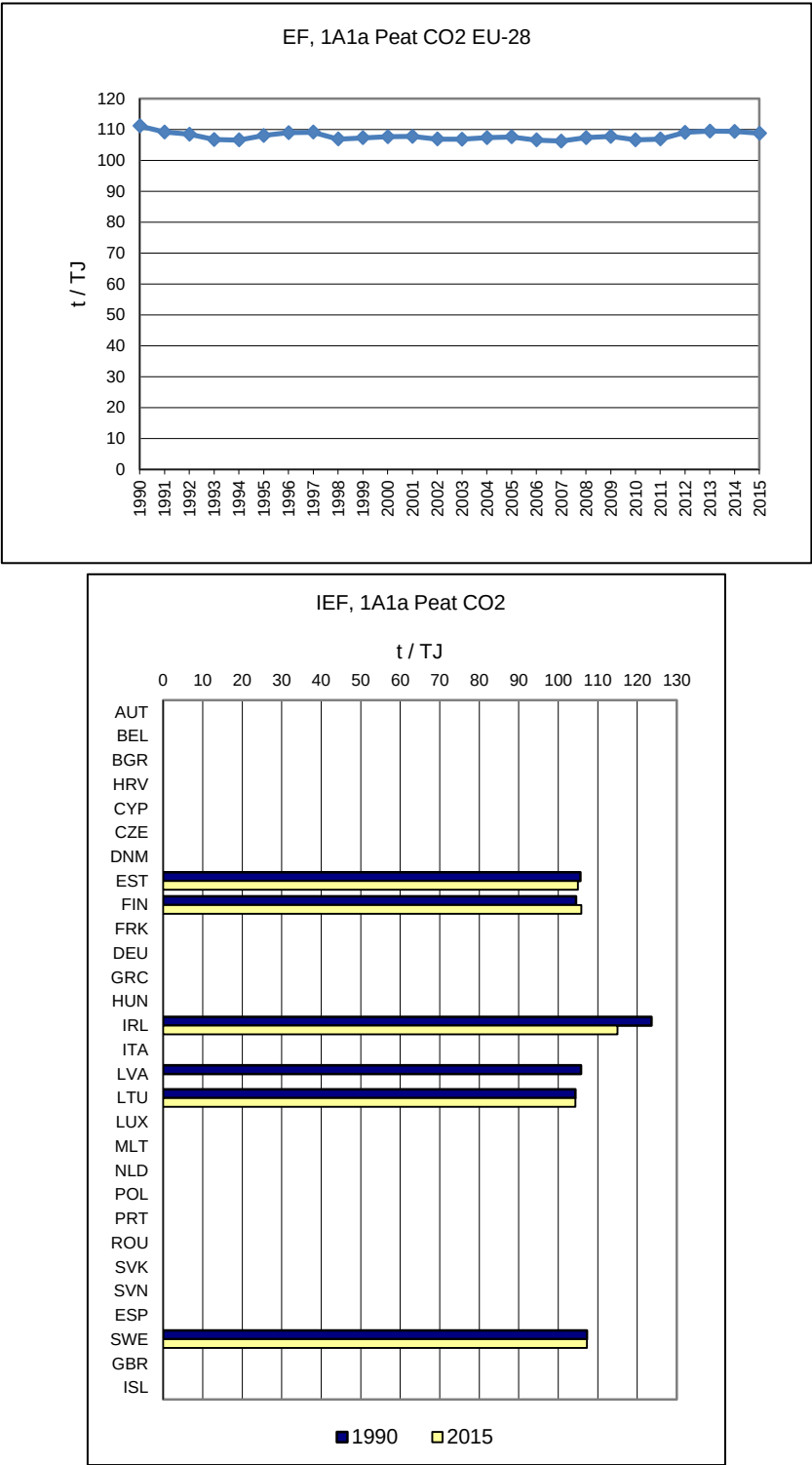
Figure 3.18 1A1a Public Electricity and Heat Production, Peat: Implied Emission Factors for CO 2
