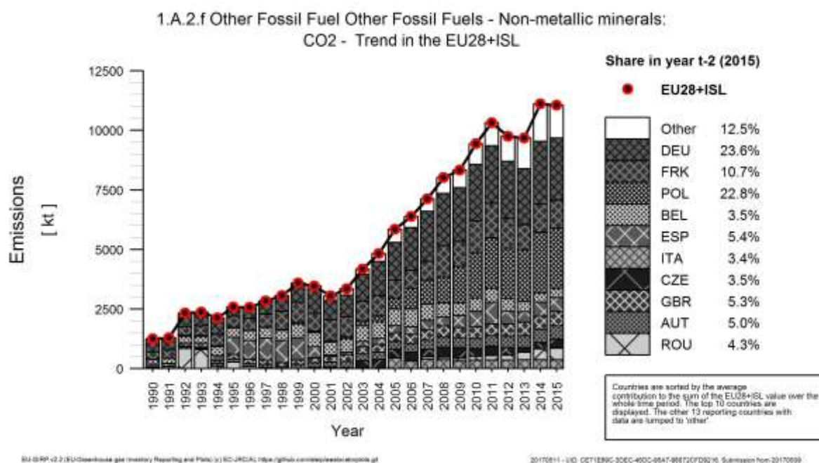
Figure 3.77 1A2f Non-metallic Minerals, other fossil fuels: Emission trend and share for CO 2
