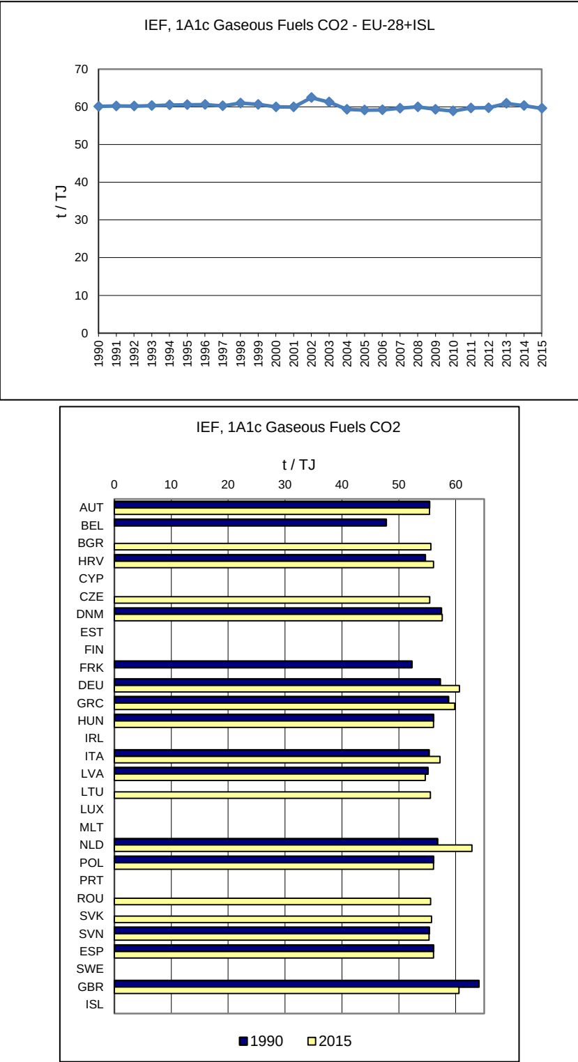
Figure 3.33 1A1c Manufacture of Solid Fuels and Other Energy Industries, Gaseous Fuels: Implied Emission Factors for CO 2
