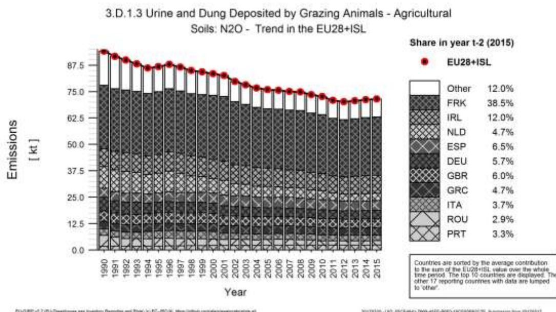
Figure 5.65: 3.D.1.3 - Urine and Dung Deposited by Grazing Animals: Trend in emissions in the EU28+ISL and the countries contributing most to EU28+ISL values including their share to EU28+ISL emissions in 2015
