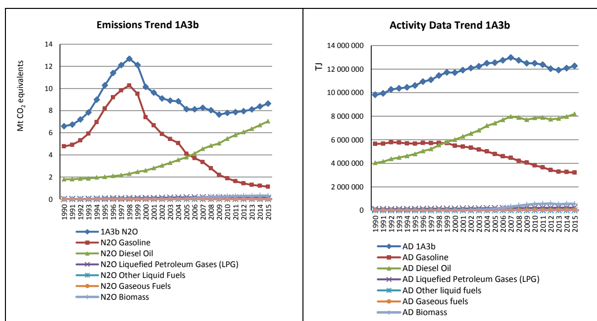
Figure 3.105 1A3b Road Transport: N 2 O Emissions Trend
