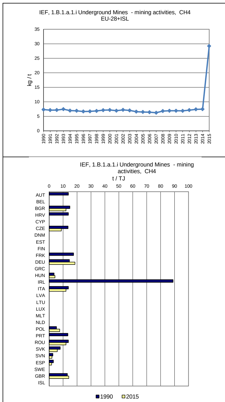
Figure 3.162: 1B1a1i Mining activities – Underground mines - Implied Emission Factors for CH 4 (in kg/t)
