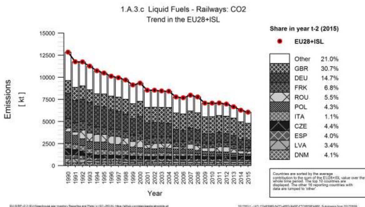
Figure 3.115 1A3c Railways, Liquid Fuels: Emission trend and share for CO 2
