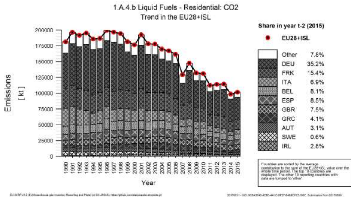
Figure 3.135 1A4b Residential, liquid fuels: Emission trend and share for CO 2
