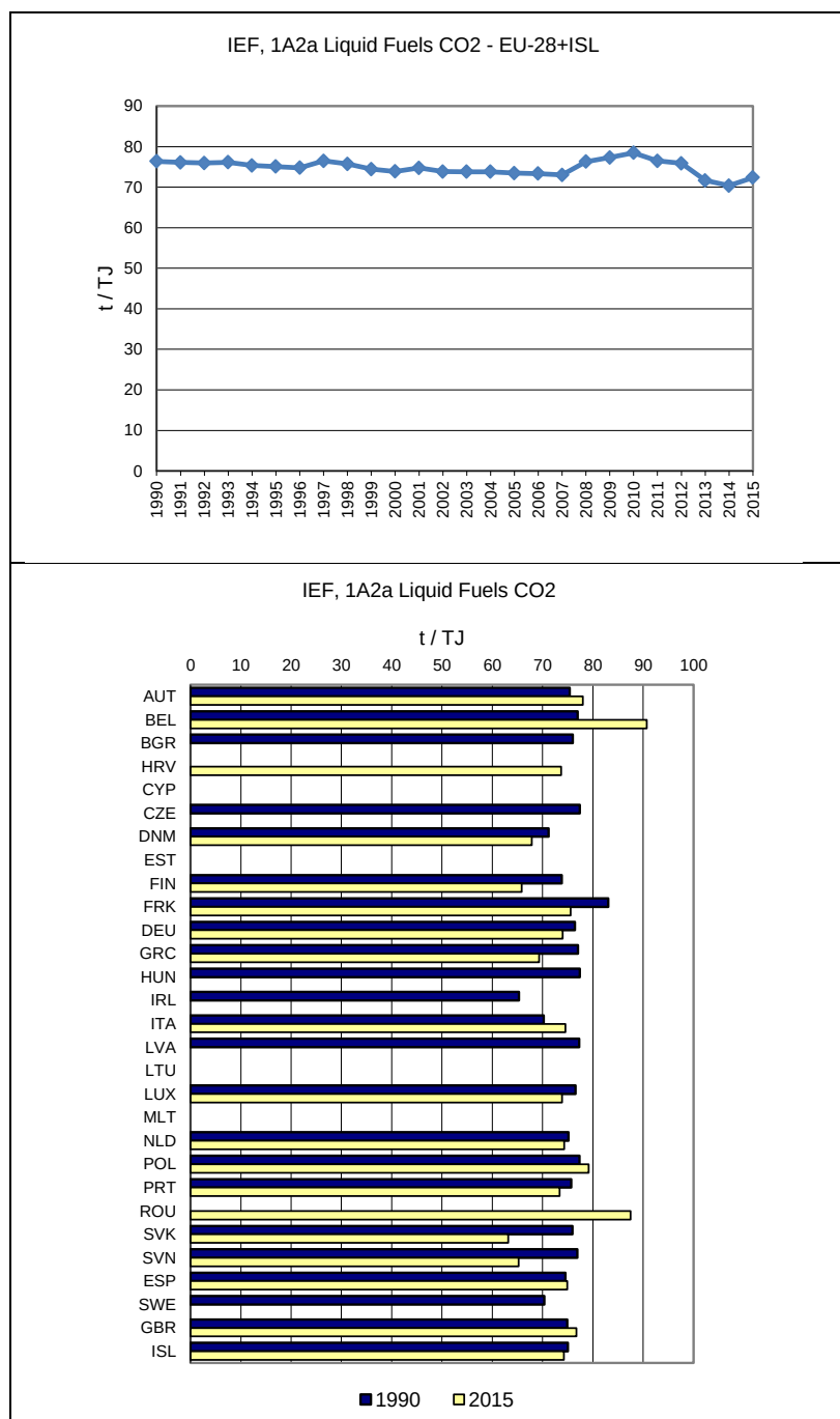
Figure 3.37 1A2a Iron and Steel, Liquid fuels: Implied Emission Factors for CO 2 (in t/TJ)
