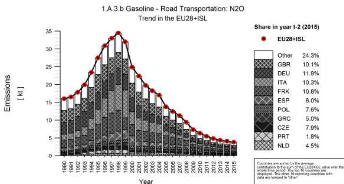
Figure 3.110 1A3b Road Transport, Gasoline: Emission trend and share for N 2 O emissions
