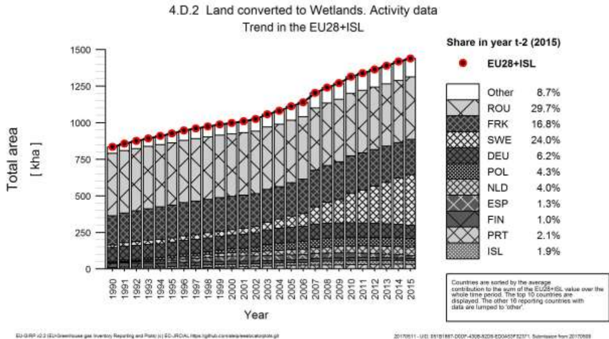
Figure 6. 16 Trend of activity data and emissions (+) / removals (-) in subcategory 4D2 “Lands converted to Wetlands” in EU MS and Iceland (kha, Kt CO2, 1990-2015)
