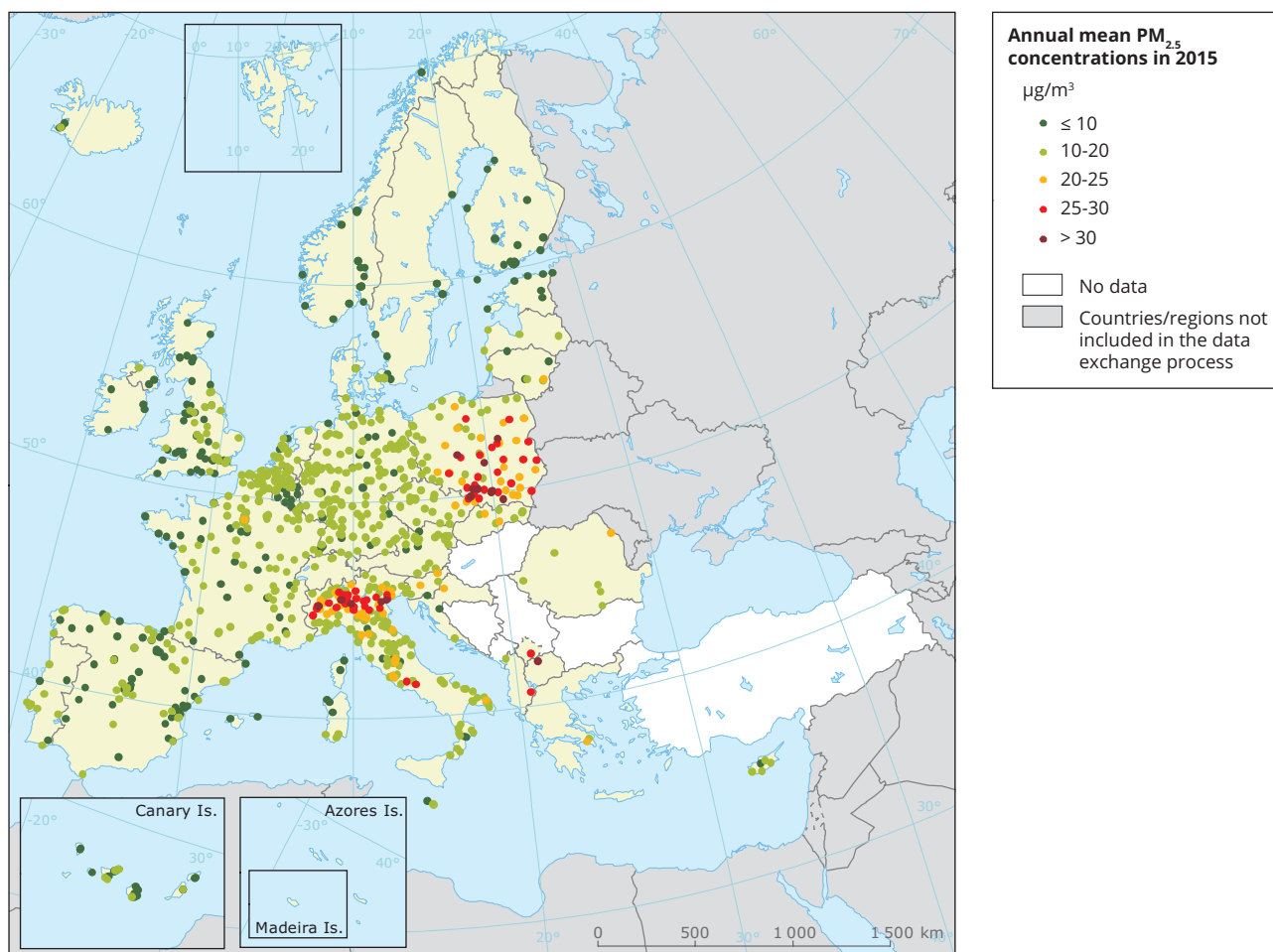
Map 4.3 Concentrations of PM 2.5 , 2015
