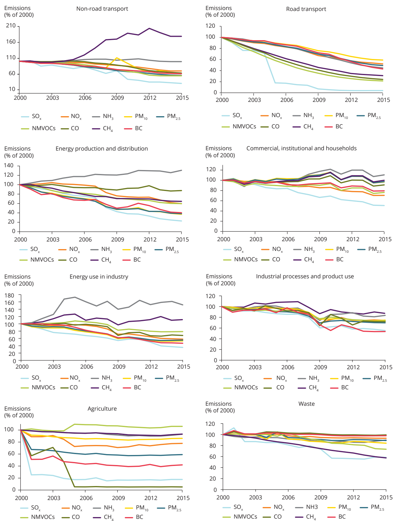
Figure 2.2 Development in EU-28 emissions from main source sectors of SO x , NO x , NH 3 , PM 10 , PM 2.5 , NMVOCs, CO, CH 4 and BC, 2000-2015 (% of 2000 levels)
