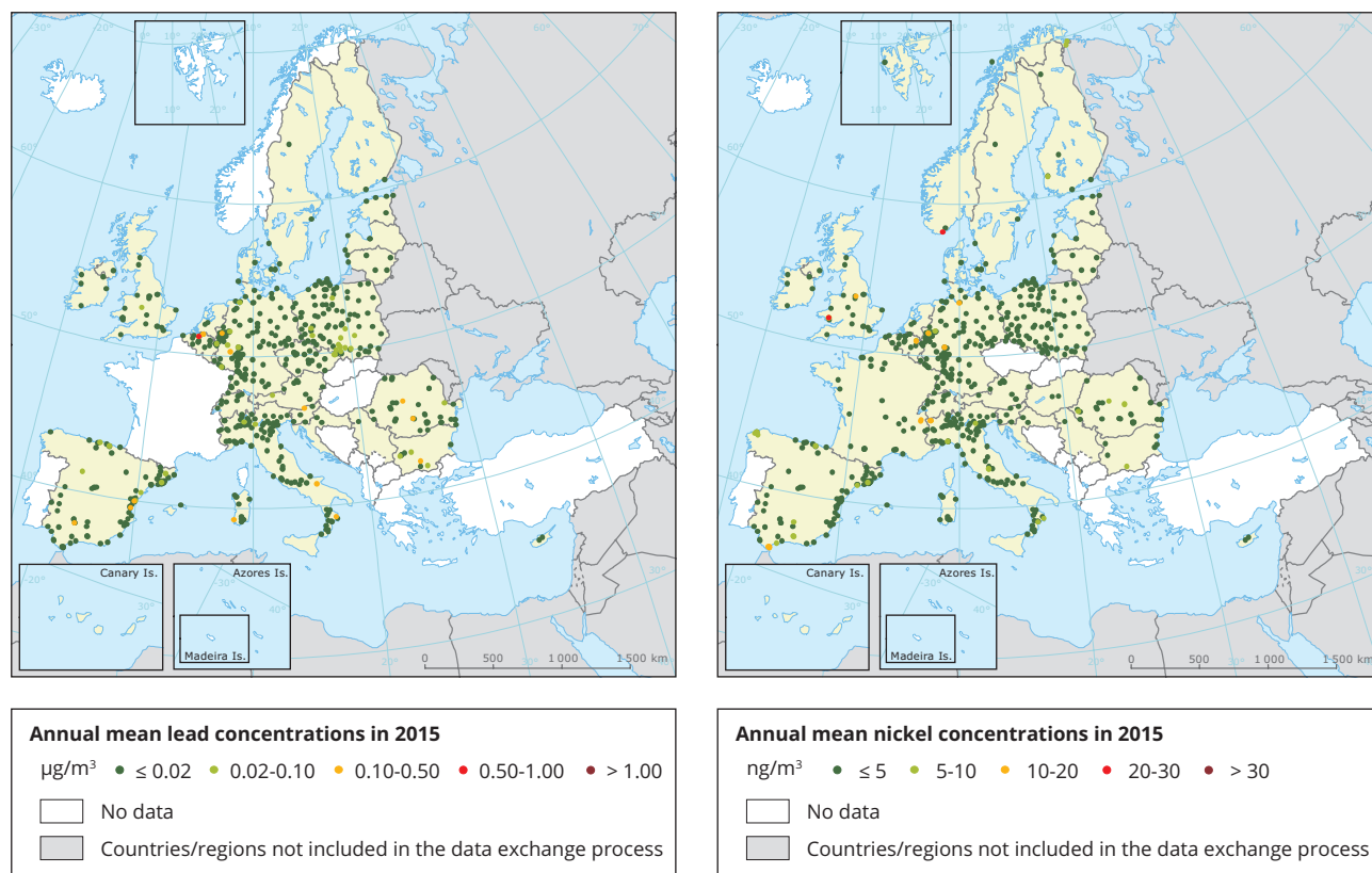
Map 8.4 Concentrations of lead and nickel, 2015
