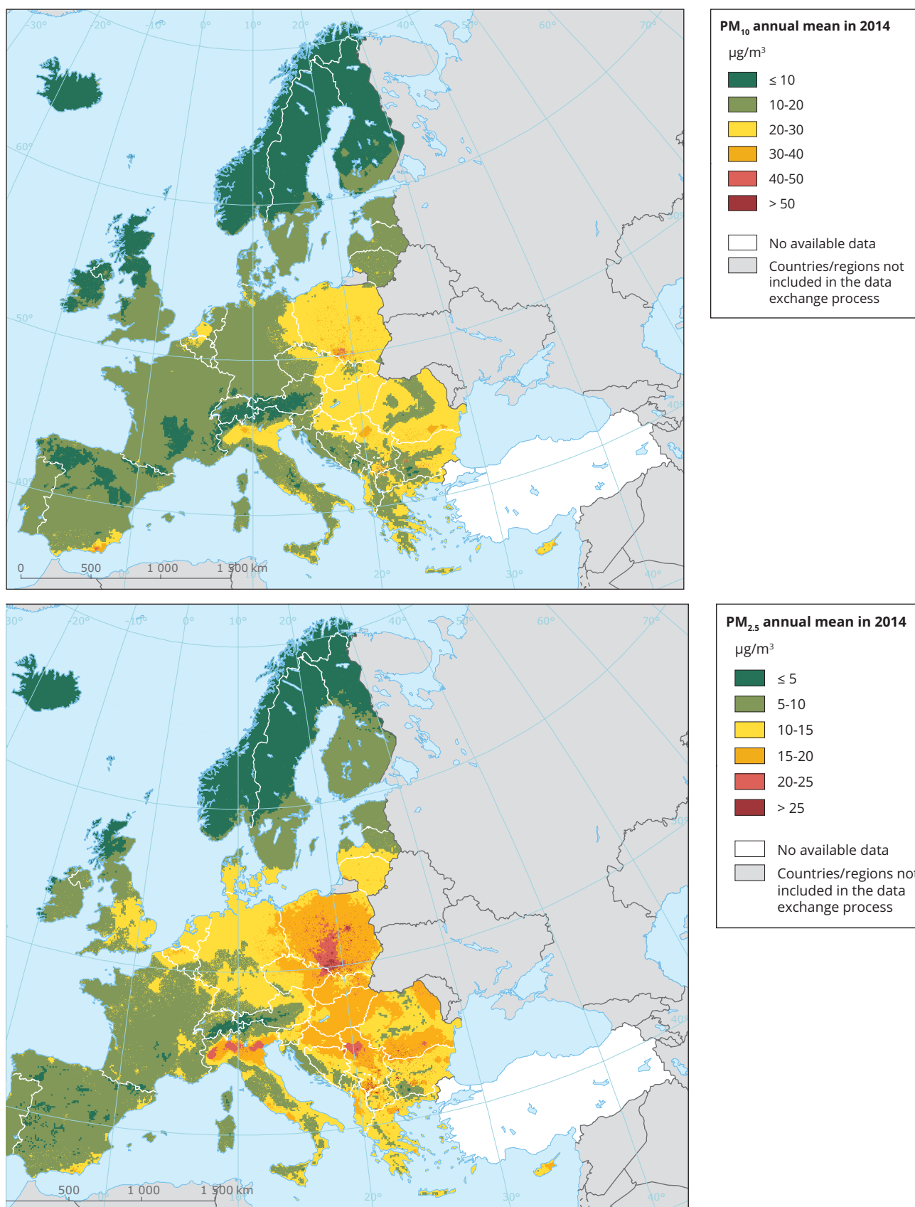
Figure 9.1 Concentration interpolated maps of PM 10 (annual mean, µg/m 3 ), PM 2.5 (annual mean, µg/m 3 ), NO 2 (annual mean, µg/m 3 ), and O 3 (SOMO35, µg/m 3 .days) for the year 2014
