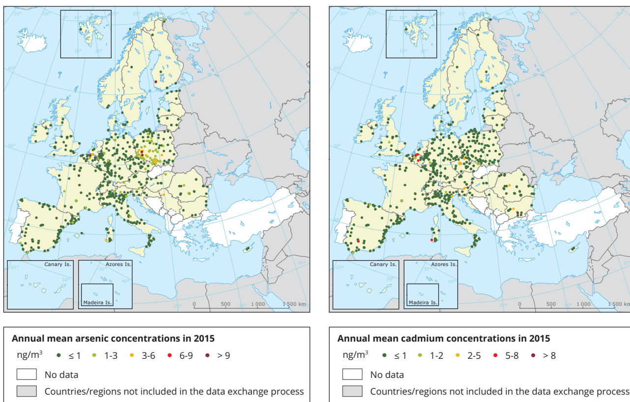
Map 8.3 Concentrations of arsenic and cadmium, 2015
