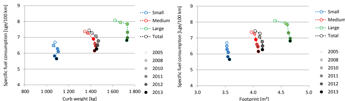
Figure 31 • Average new LDV fuel economy by segment over vehicle weight and footprint, 2013
