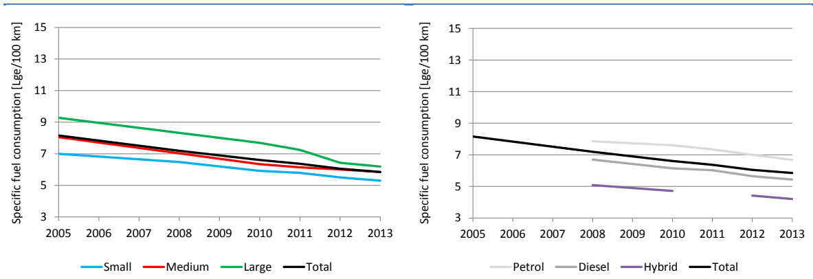
Figure 60 • Average new LDV fuel economy by vehicle segment and powertrain, 2005-13
