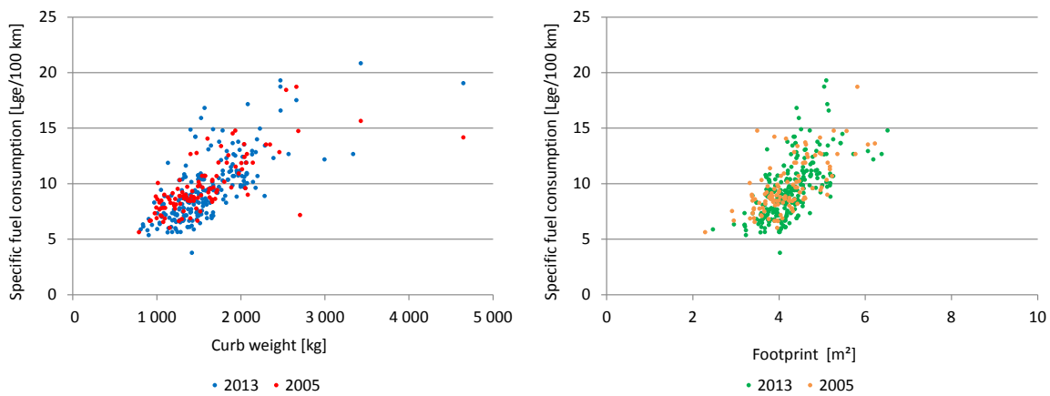
Figure 45 • Fuel economy of new LDVs over vehicle weight and footprint, 2005 and 2013
