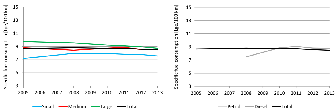
Figure 21 • Average new LDV fuel economy by vehicle segment and powertrain, 2005-13
