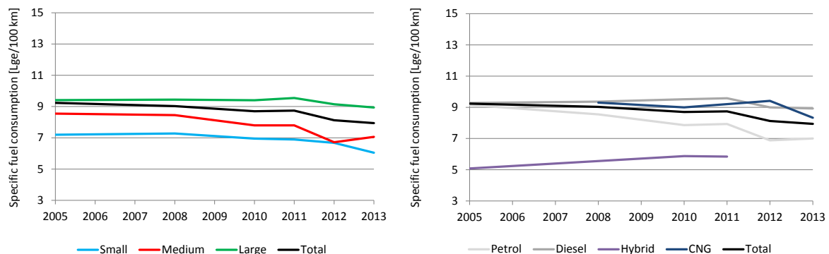
Figure 56 • Average new LDV fuel economy by vehicle segment and powertrain, 2005-13
