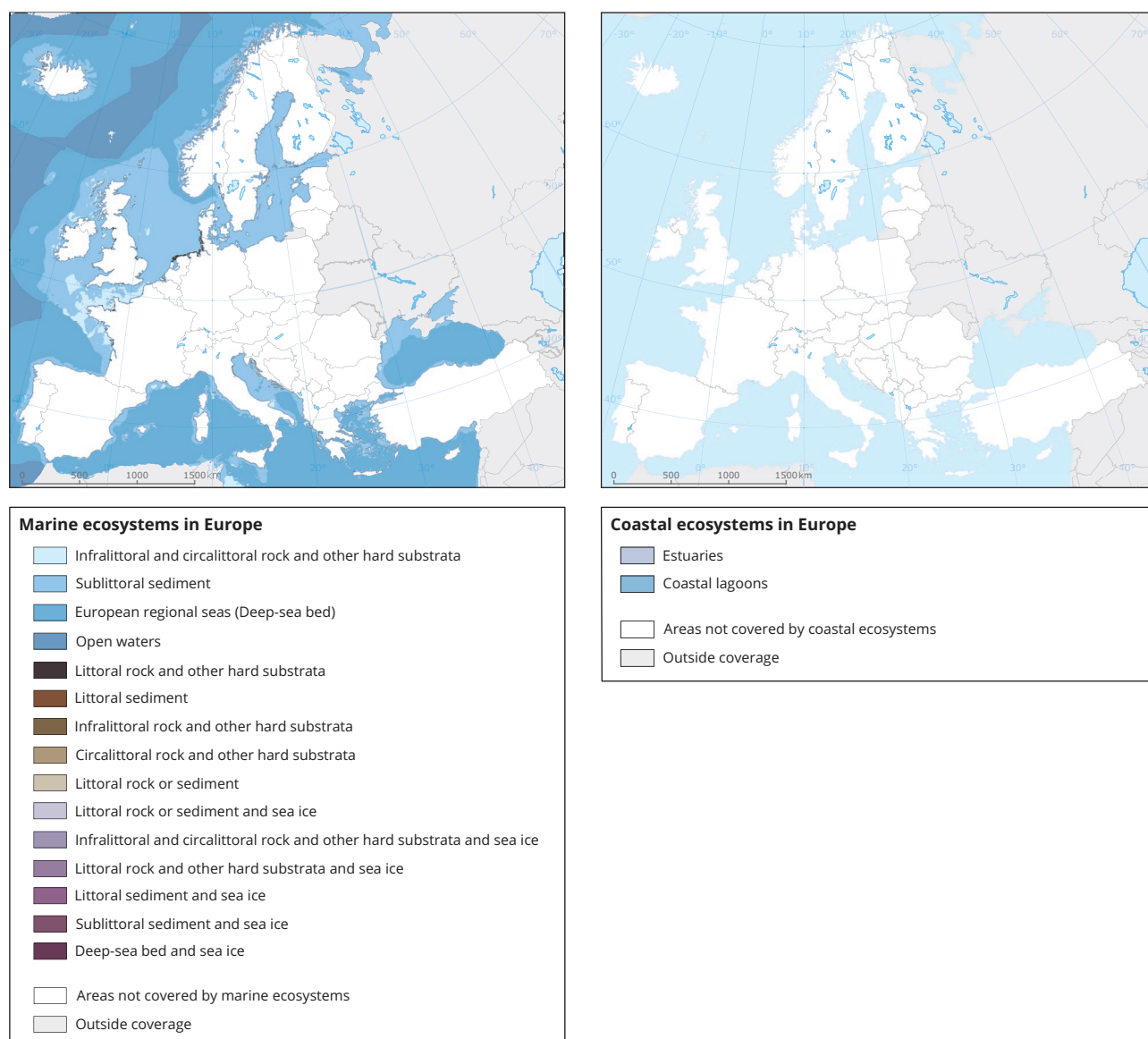
Map 5.28 Marine ecosystems in Europe
