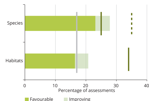
Figure 5.18 Progress to the 2020 target for habitats and species assessed under the Habitats Directive
