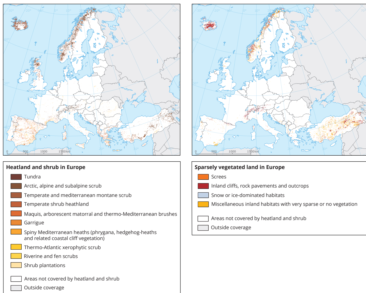
Map 5.19 Heathland and shrub (left) and sparsely vegetated land (right) in Europe
