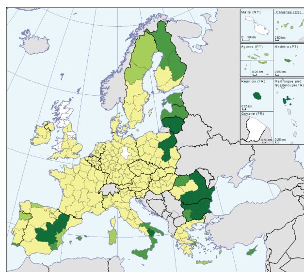
Map 5.7 Share of utilised agriculture land for extensive arable crop
