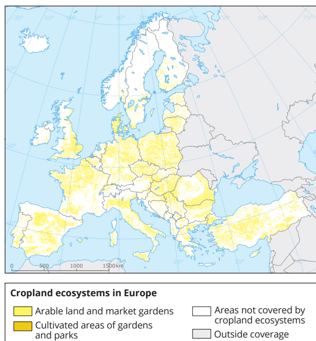
Map 5.5 Cropland ecosystems in Europe
