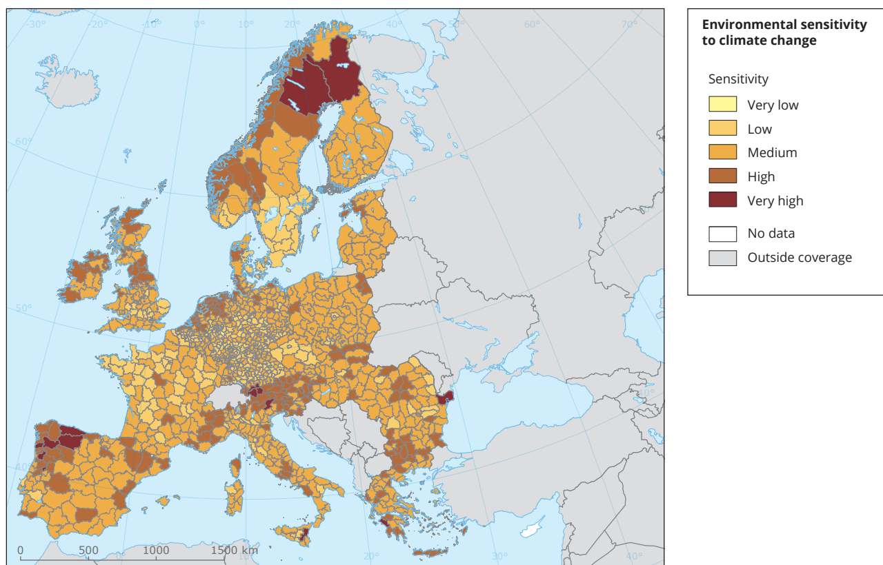
Map 4.3 Environmental sensitivity to climate change
