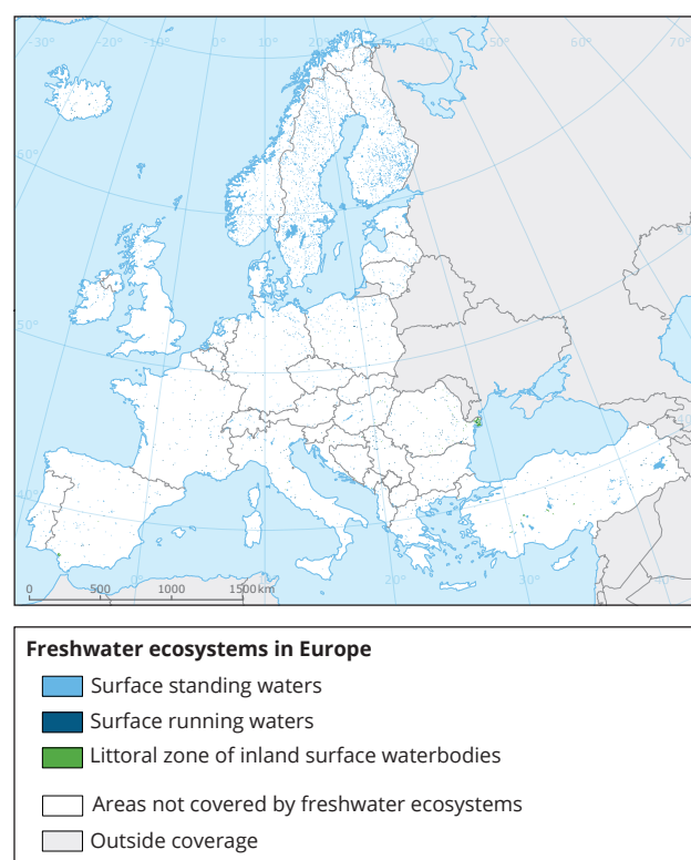
Map 5.23 Freshwater ecosystems in Europe
