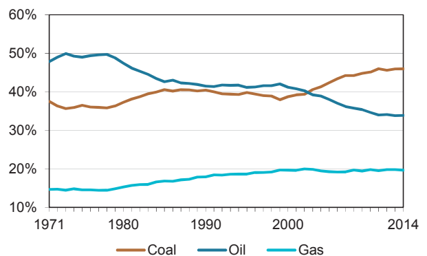
Figure 7. Fuel shares in global CO 2 emissions
