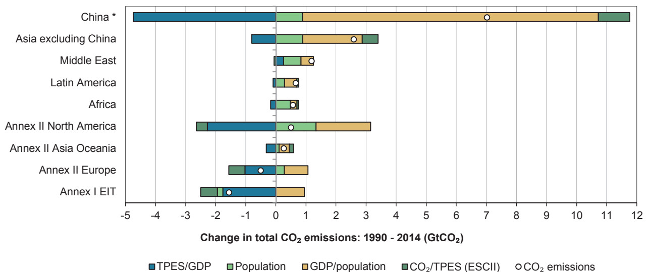
Figure 19. Global CO 2 emissions and drivers (Kaya decomposition): 1990-2014 3
