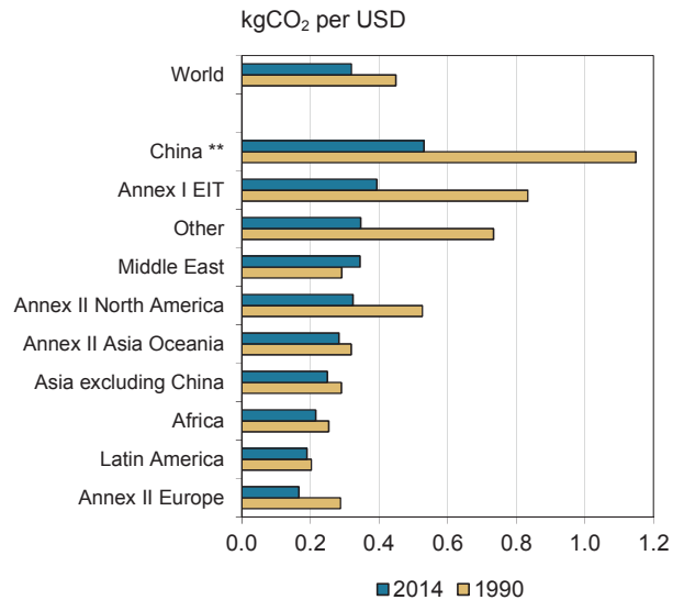
Figure 16 CO 2 emissions per GDP* by major world regions
