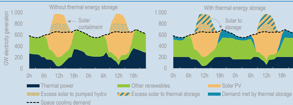
Figure 3.20 • Illustrative analysis of the potential role of storage using solar PV for district cooling over two days in April 2050 during the peak cooling period in India
